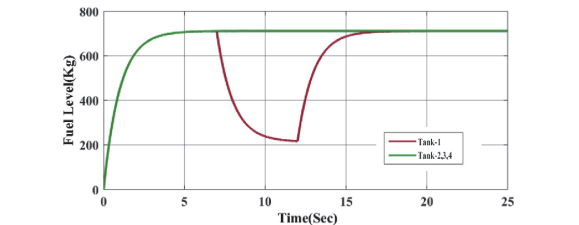
Figure 17. Fuel management test without a controller.
