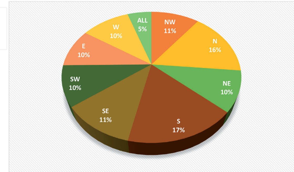
Figure 2. Distribution of landslide areas according to directions.
