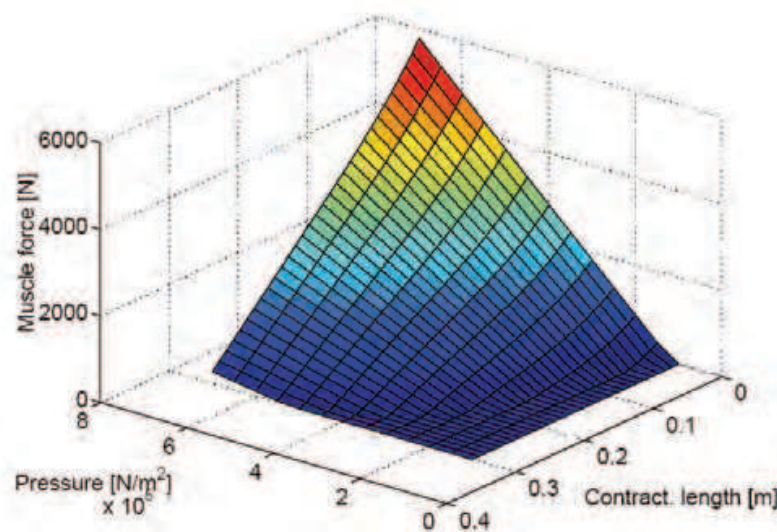
Fig. 6. Force characteristic of a pneumatic muscle.
