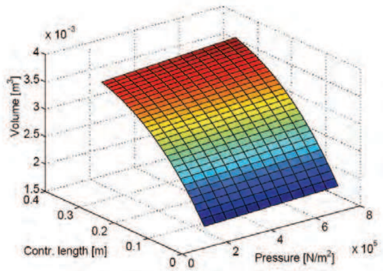
Fig. 5. Volume characteristic of a pneumatic muscle.
