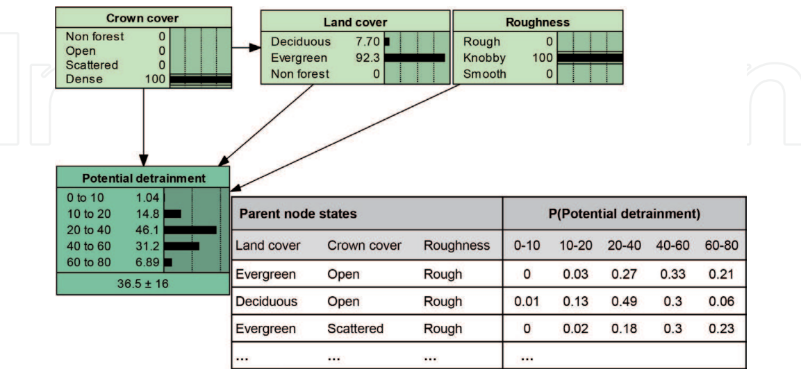
Figure 1. Example of a Bayesian Network for potential braking effect of the forest during avalanches (detrainment of snow), which is a child node of the parent nodes crown cover, land cover, and terrain roughness, with the corresponding conditional probability table, which contains the probability distribution of potential detrainment for each combination of its parent nodes. In this example, the states of the nodes “crown cover” and “roughness” are known with 100% certainty, while “land cover” is known with some uncertainty, and this information propagates to the other nodes in the network.
