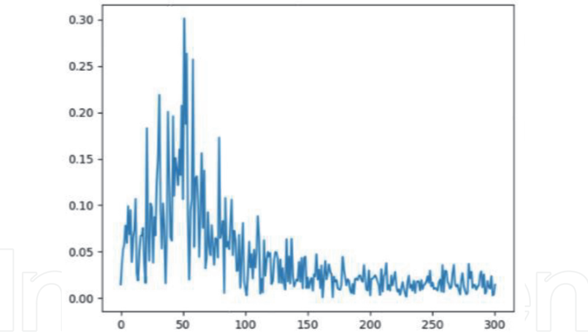
Figure 13. FFT plot with imbalance load on the motor.
