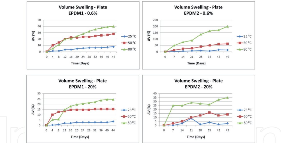
Figure 15. Volume swelling of plate samples; low and high salinities; different temperatures.
