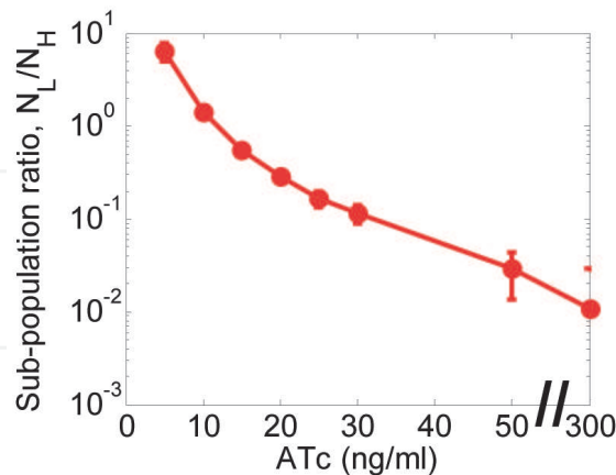
Figure 1. (A) Schematic of the positive feedback (PF) synthetic gene circuit in yeast (top left). The regulator rtTA is toxic when active, but the gene circuit prevents Zeocin toxicity by activating the ZeoR gene (top right). The role of cellular memory in optimizing fitness is shown in the bottom panel. (B-E) dose responses. (B) Mean expression levels of the PF gene circuit and of the cell sorted low- and high-expression states. (C) Gene expression noise as determined from the coefficient of variation (CV). (D) Subpopulation ratio of low-expressing cells to high-expressing cells. (E) Steady-state gene expression distributions at a single-cell resolution. From Figure 2 “characterization of gene expression in cells bearing PF circuit” by Nevozhay, D. and Adams, R. et al. in [25] located at https://journals.plos.org/ploscompbiol/article?id=10.1371/journal.pcbi.1002480 under a CC BY 4.0 license with panel label font modified.
