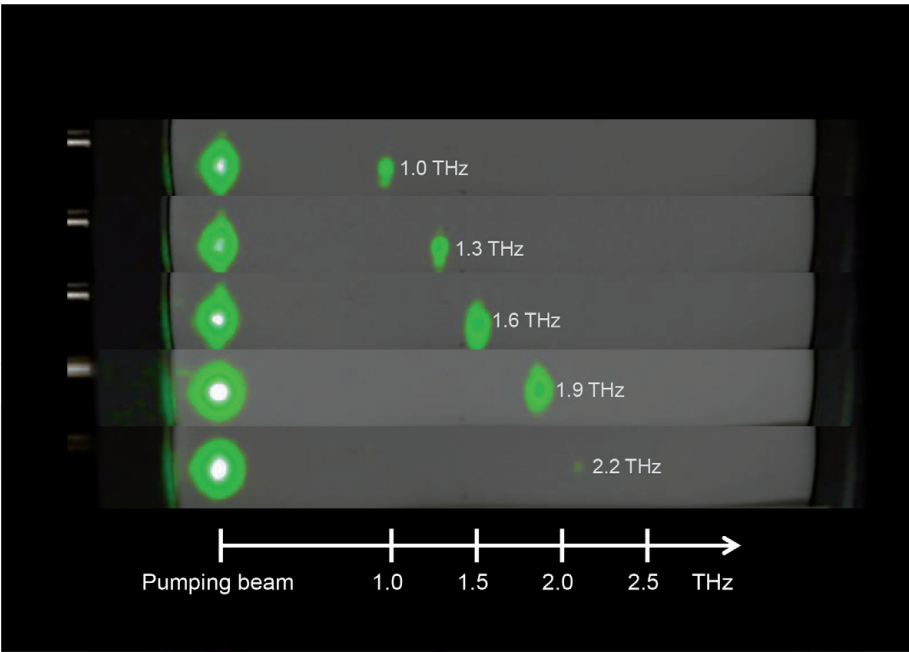
Figure 5. Pictures of the up-converted signals on the laser beam visualizer when the input frequency of terahertz wave of 1.0, 1.3, 1.6, 1.9 and 2.2 THz.
