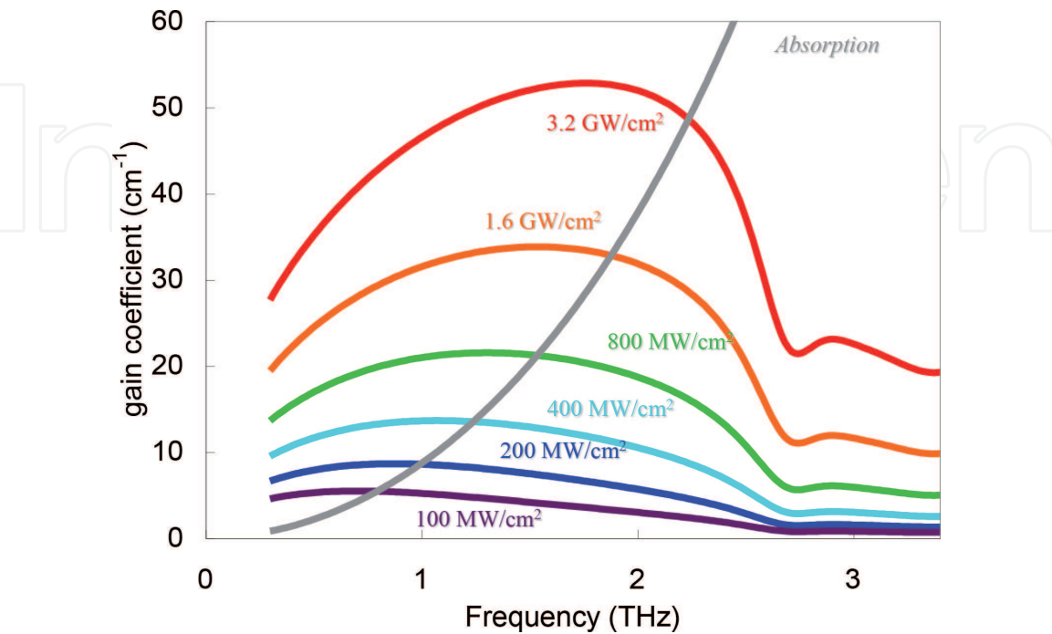
Figure 3. Calculated gain and absorption coefficient using MgO:LiNbO 3 pumped by Nd:YAG laser for several pumping intensities, 0.1, 0.2, 0.4, 0.8, 1.6, and 3.2 GW/cm 2 .
