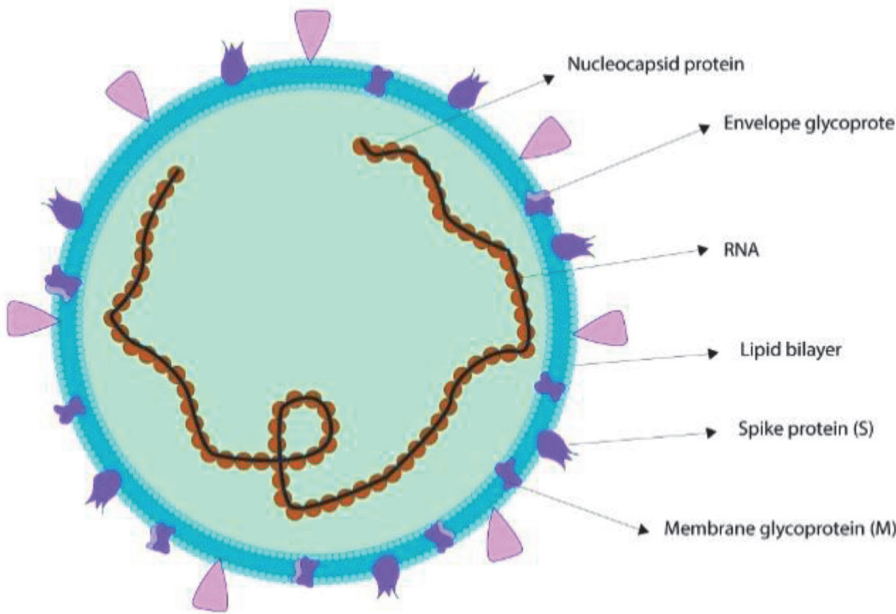
Figure 3. Structure of the coronavirus (Sars-CoV2) [63].
