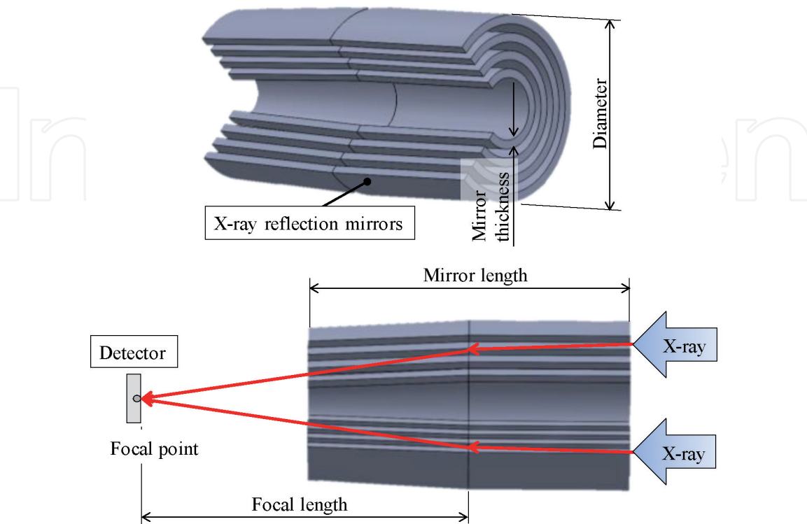
Figure 1. Structure of the X-ray telescope structure [1].
