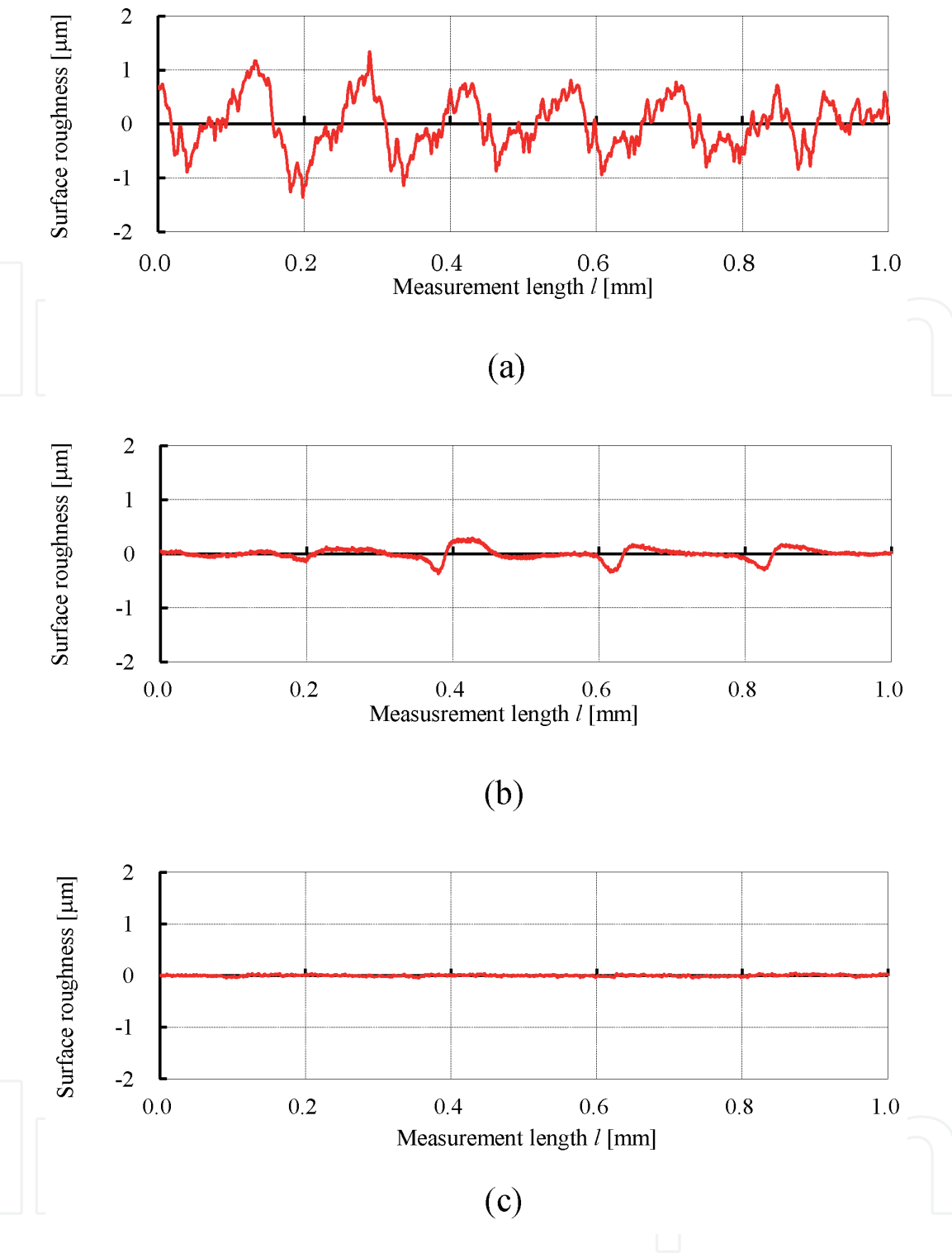
Figure 6. Surface roughness of polished SUS310S surface. (a) before polishing [ Ra = 0.40 \mu m , Rz = 2.70 \mu m ]. (b) after 1 hour polishing [ Ra = 0.07 \mu m , Rz = 0.66 \mu m ]. (c) after 37 hours polishing [ Ra = 0.02 \mu m , Rz = 0.15 \mu m ].
