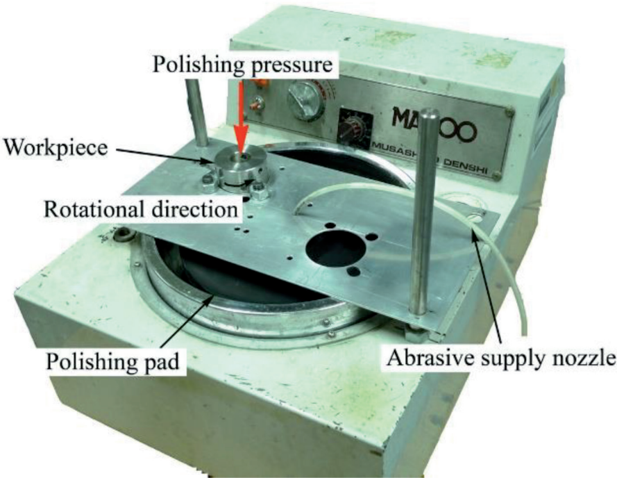
Figure 3. Overview of precision polishing machine and experiment.
