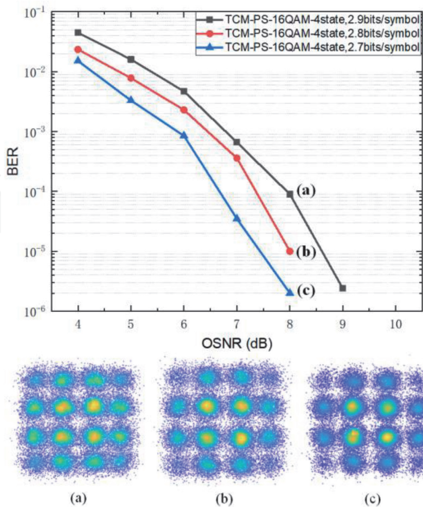
Figure 6. BER curves and constellations of TCM-PS-16QAM-4state for 25-km transmission. (a) H=2.9 bits/symbol, (b) H=2.8 bits/symbol, (c) H=2.7 bits/symbol.
