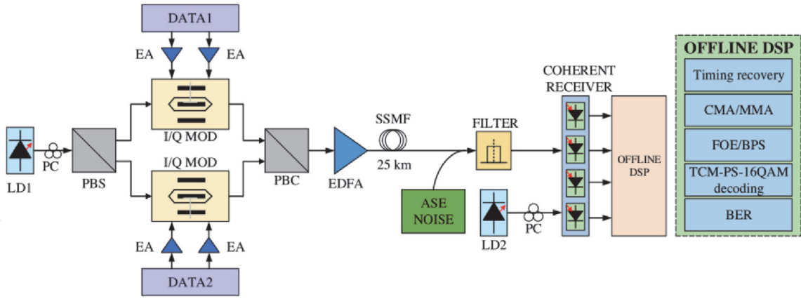
Figure 3. Experimental setup for PDM single carrier system.
