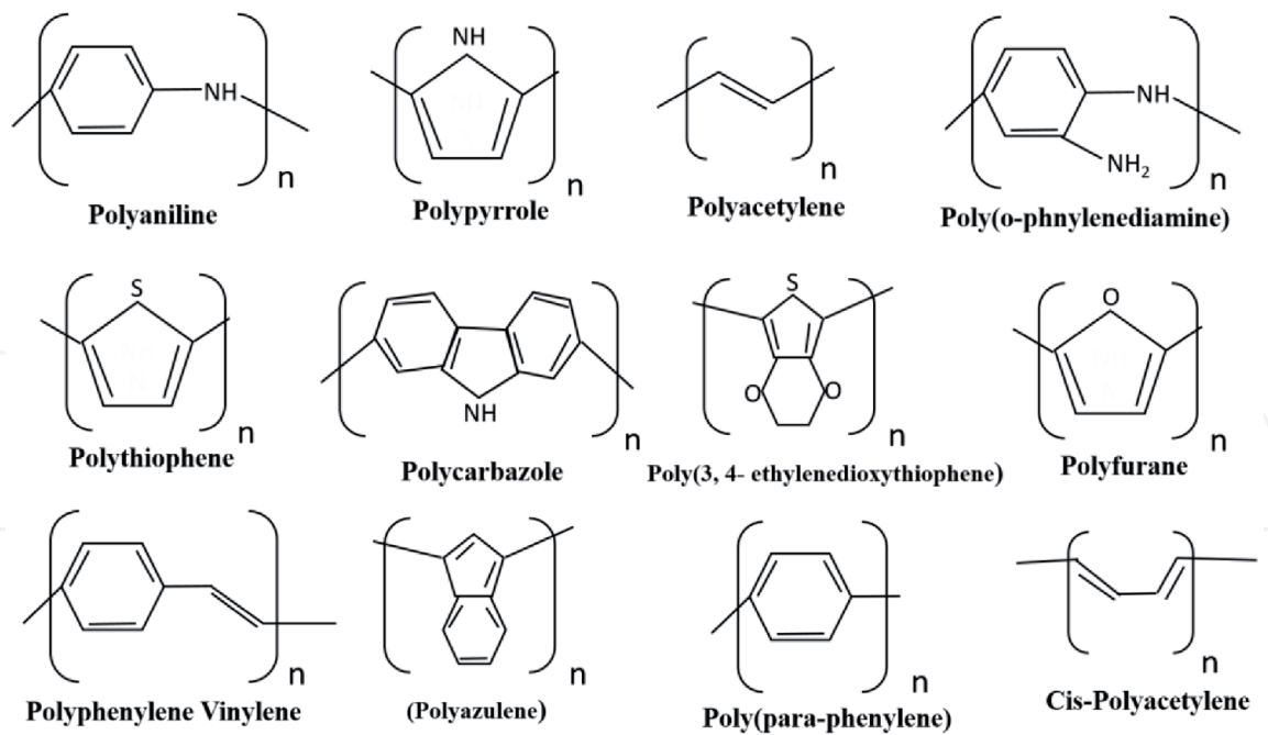
Figure 5. Chemical structure of conducting polymer [27].
