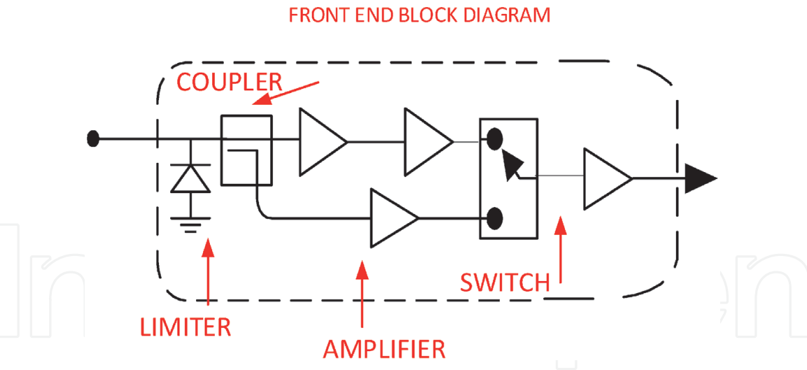
Figure 3. MM-wave frontend block diagram.
