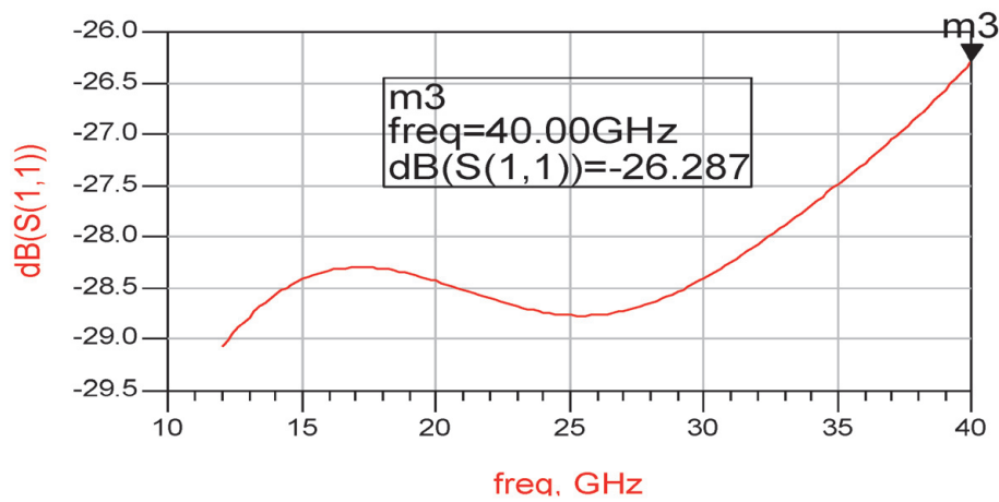
Figure 35. S11 of the wideband coupler.
