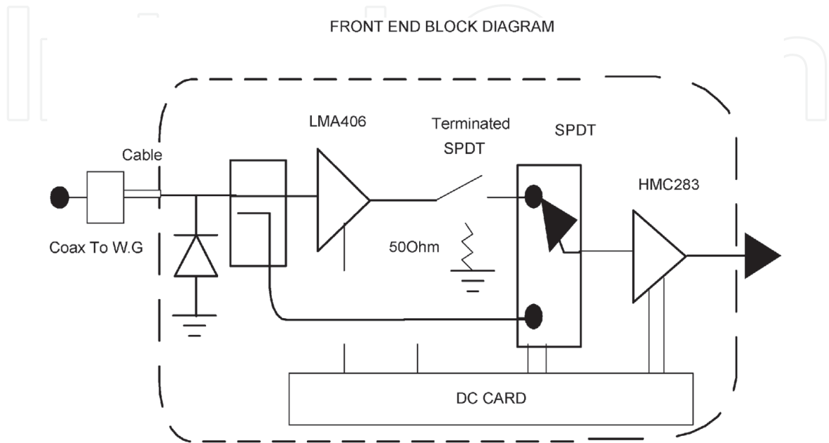
Figure 9. Block diagram of the high gain wideband frontend with one LMA406 amplifier.
