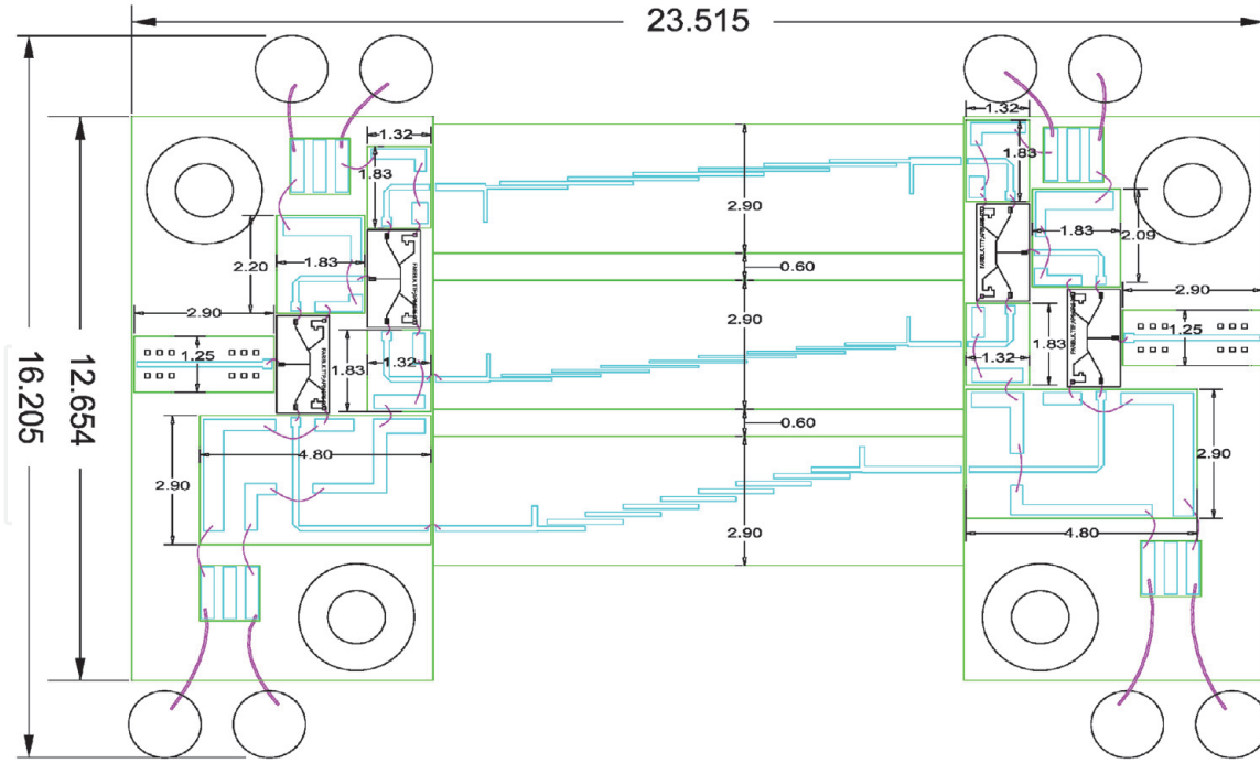
Figure 24. SFB layout.
