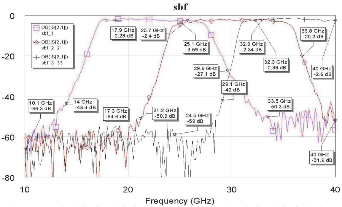
Figure 30. SFG detailed measured S_{12} results.
