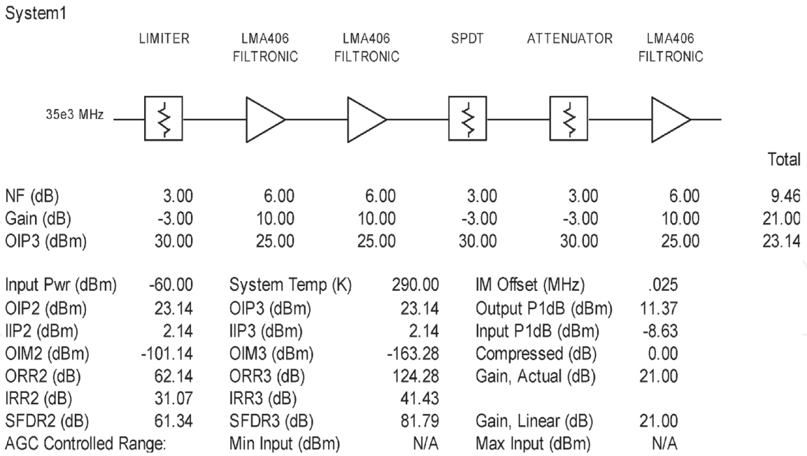
Figure 4. Frontend module design for LNA NF = 6 dB.
