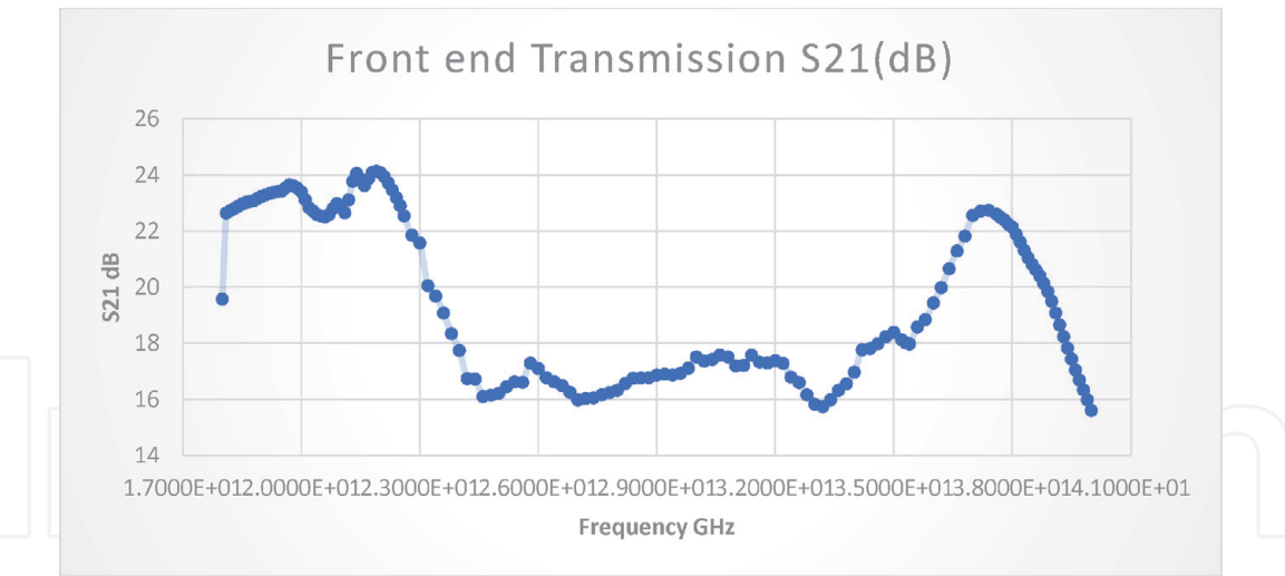
Figure 6. Measured wideband frontend gain 17 GHz to 40 GHz.
