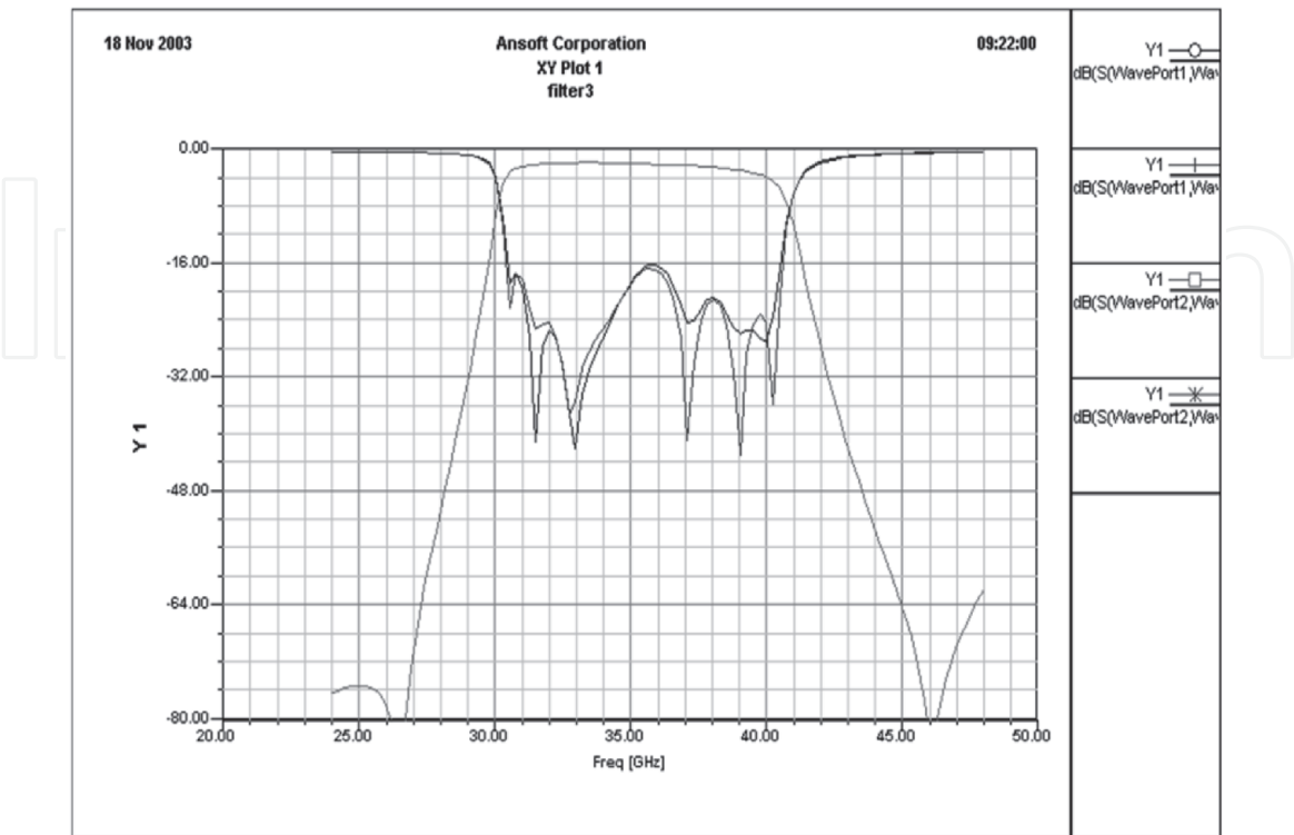
Figure 20. S parameters for filter #3.
