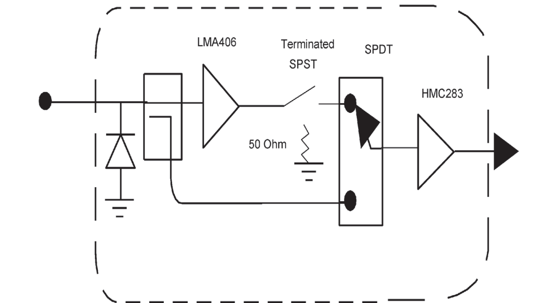
Figure 7. High gain frontend block diagram.
