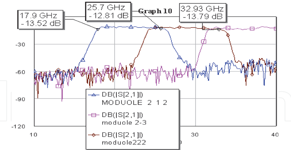
Figure 26. SFB measured results unit number 1.
