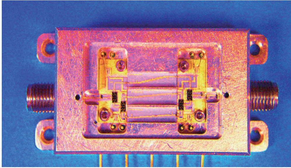
Figure 25. SFB picture.
