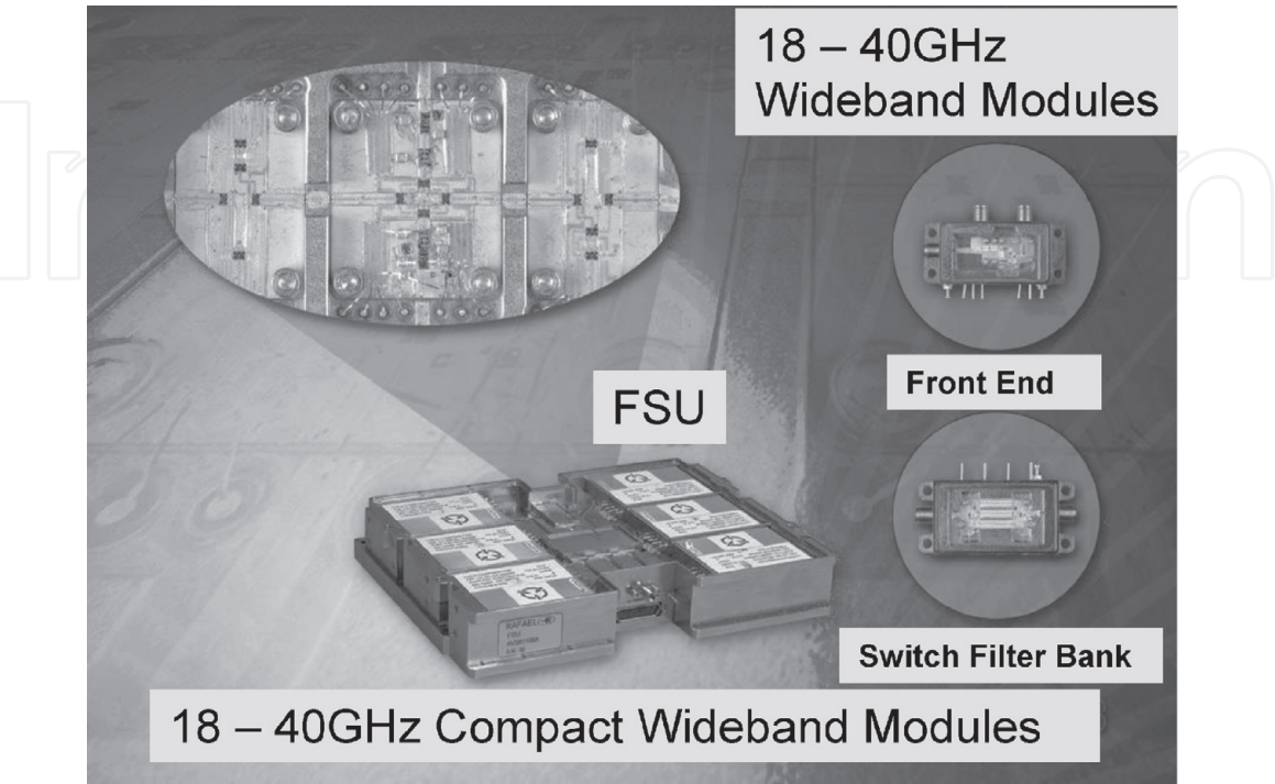
Figure 14. Photo of 18–40GHz compact modules.
