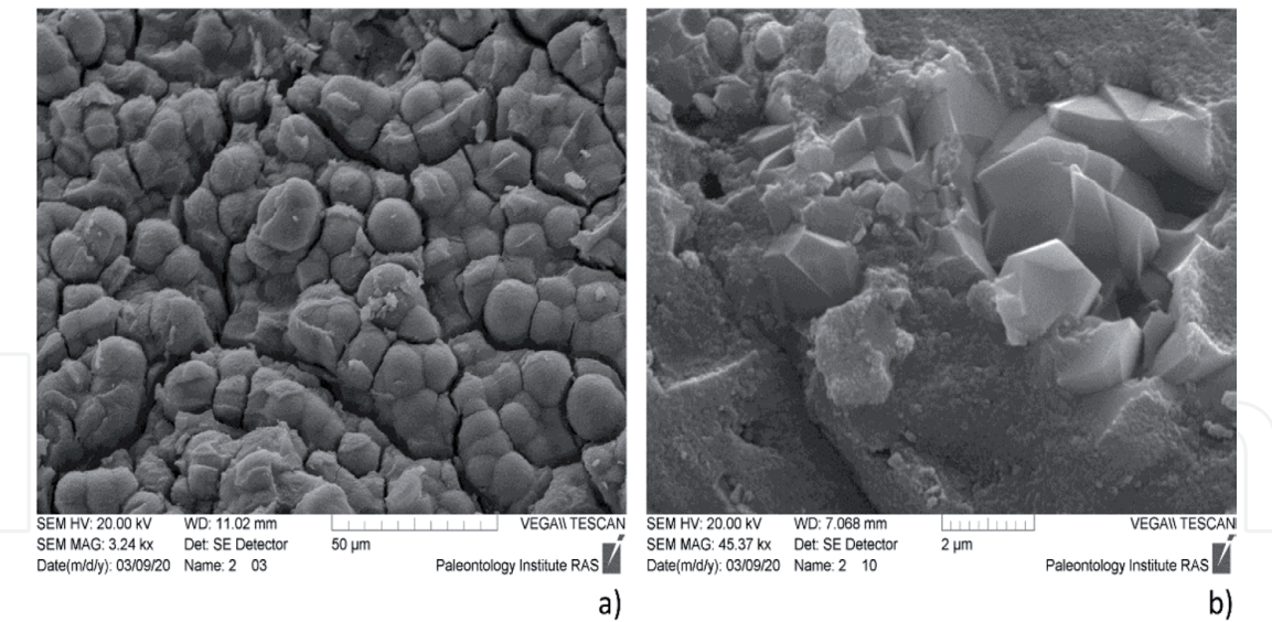
Figure 4. Micrographs of the ferromanganese crust with different magnifications: (a) numerous columns of stromatolites are seen (top view); (b) microcrystals of apatite lying on bacterial mats.
