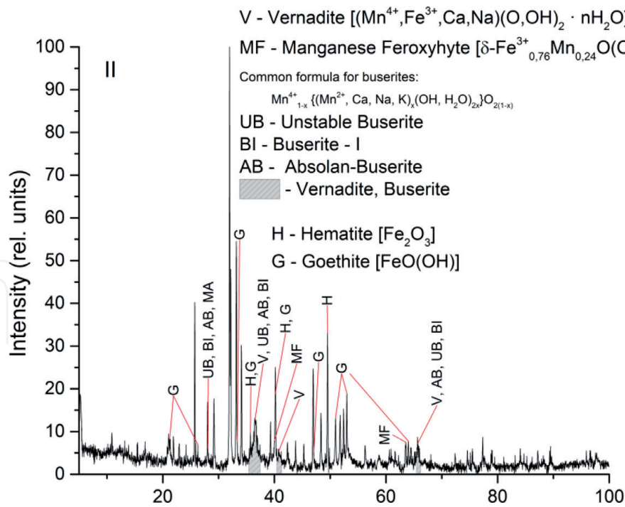
Figure 7. X-ray diffractograms of layer I-1, I-2.
