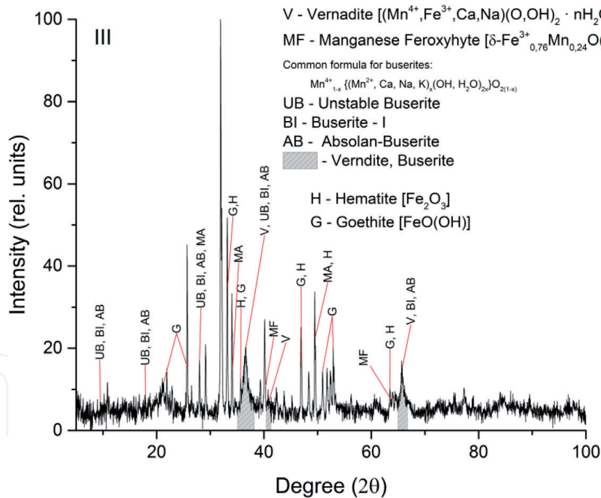
Figure 8. X-ray diffractograms of layer II, III.
