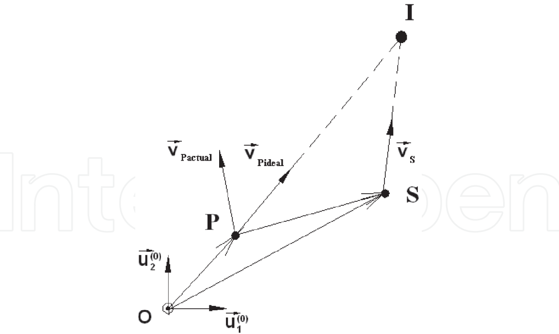
Figure 5. Linear homing guidance law geometry.
