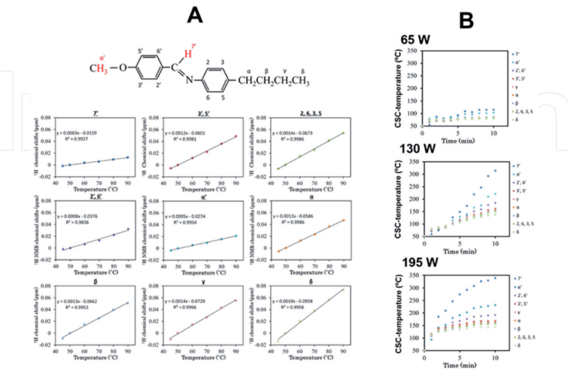
Figure 6. A. Plots of 1 H chemical shift against setting the temperature of NMR spectrometer. B. Temperature as a function of the microwave irradiation time at a microwave power of 65, 130, and 195 W [33].
