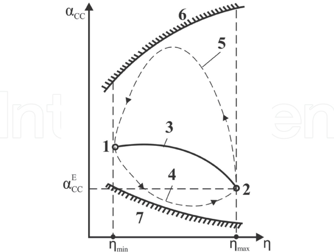
Figure 6. Typical change in excess air ratio \alpha_{cc} in the combustion chamber of a gas turbine engine when changing its operating mode.
