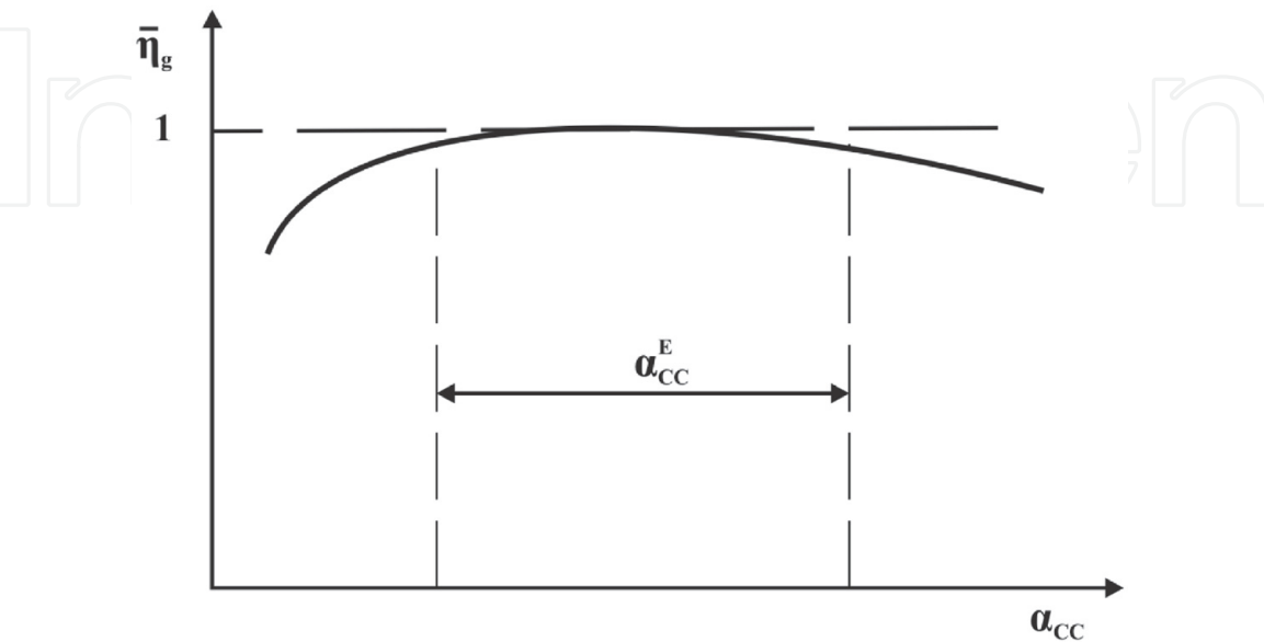
Figure 14. The characteristic of the ATCC with a self-adjusted adaptive system of regulation, where \alpha_{CC}^E – The range of calculated modes of the excess air ratio in the combustion chamber for this method of controlling the organization of the combustion process.
