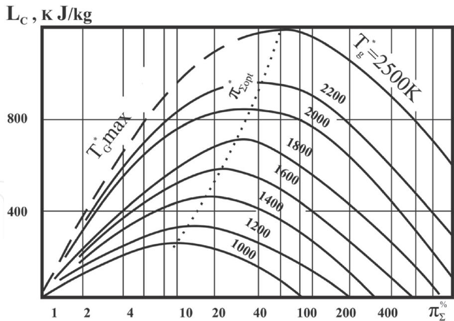
Figure 3. Dependence of the cycle L_C from \pi_{\Sigma}^* if T_G^* = \text{var.} and T_H^* = \text{const.}
