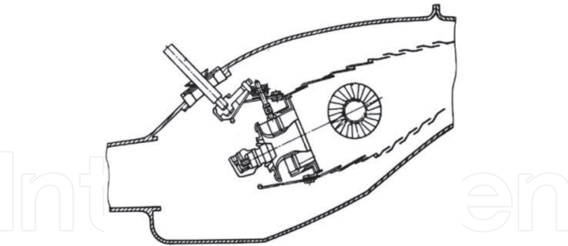
Figure 11. The possible CC scheme with an adjustable head.
