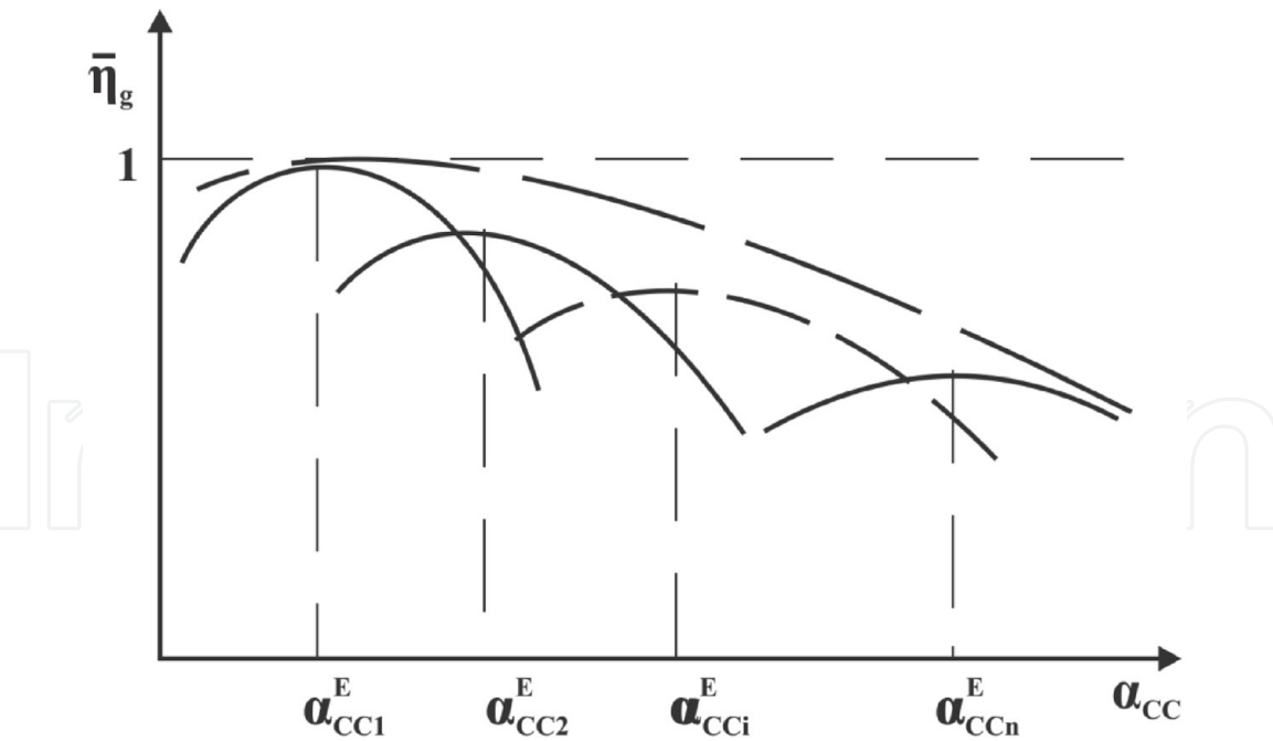
Figure 13. Graphical characteristic of the ATCC with an adaptive choice of options.
