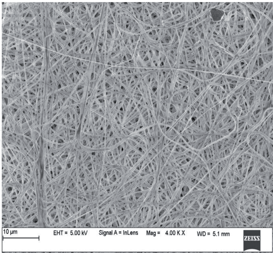
Figure 4. SEM image of the PVA-HA film, scale 10 μm and 4K X magnification.
