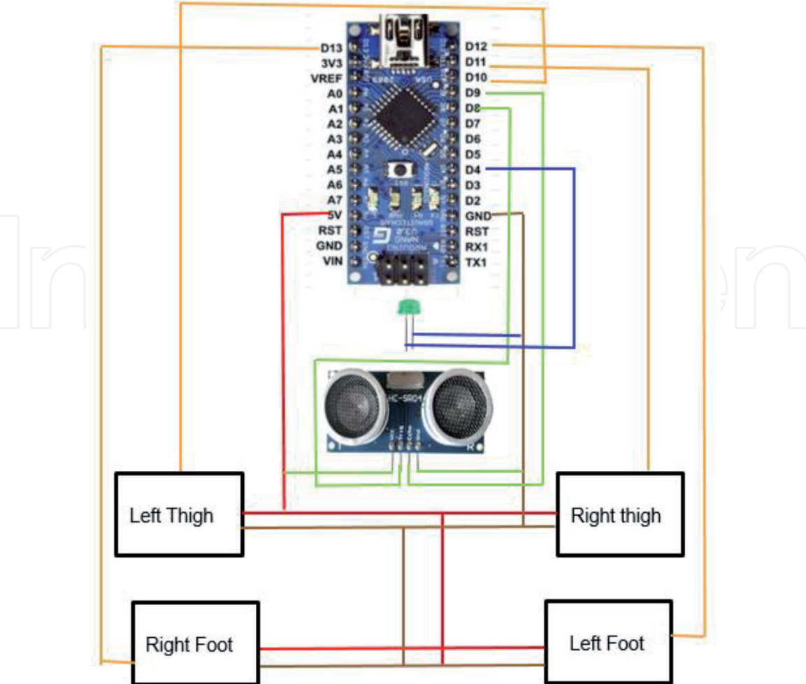
Figure 3. Connection structure of tiny humanoid.
