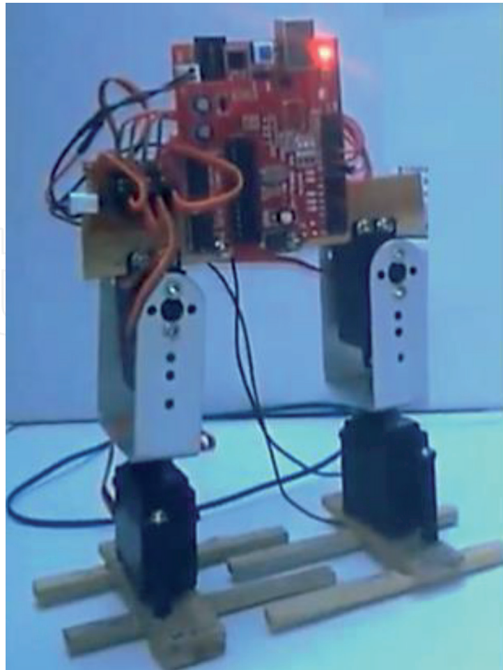
Figure 2. Humanoid robot (autonomous) using Arduino.
