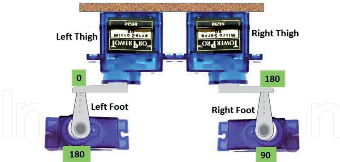
Figure 4. Turning values of servo horns.
