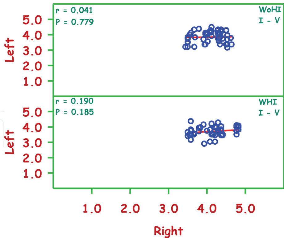
Figure 6. Correlation of IPL I-V (ms) in type 2 diabetes, without (WoHI) and with (WHI) hearing impairment. n = 50 each. The 'r' and P values are correlating WoHI and WHI right and left ear.
