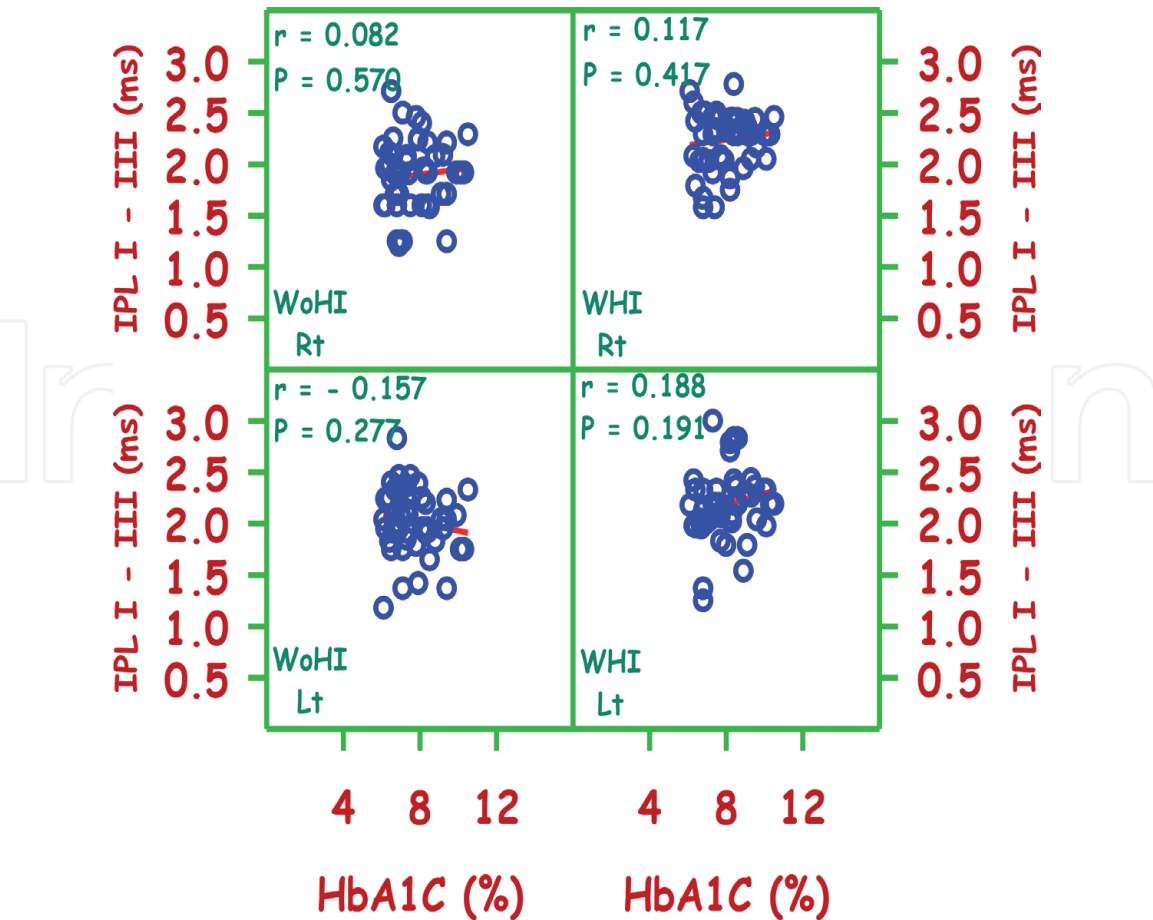
Figure 13. Correlation of IPL I-III and HbA1c in type 2 diabetes, without (WoHI) and with (WHI) hearing impairment. The 'r' and P values are correlating WoHI and WHI right and left ear.
