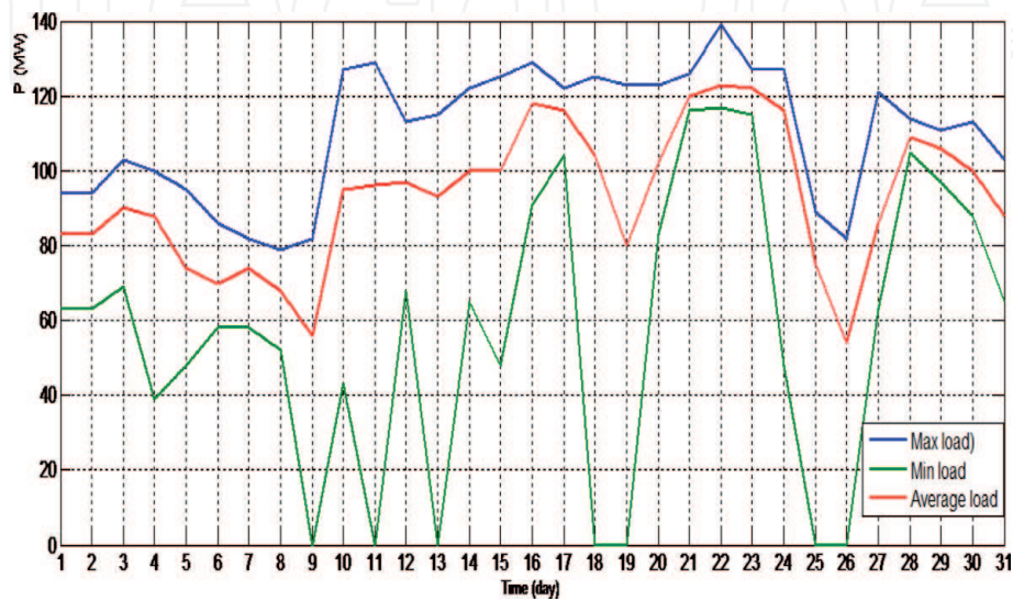
Figure 15. The performance of GT14 in Aug-2020.
