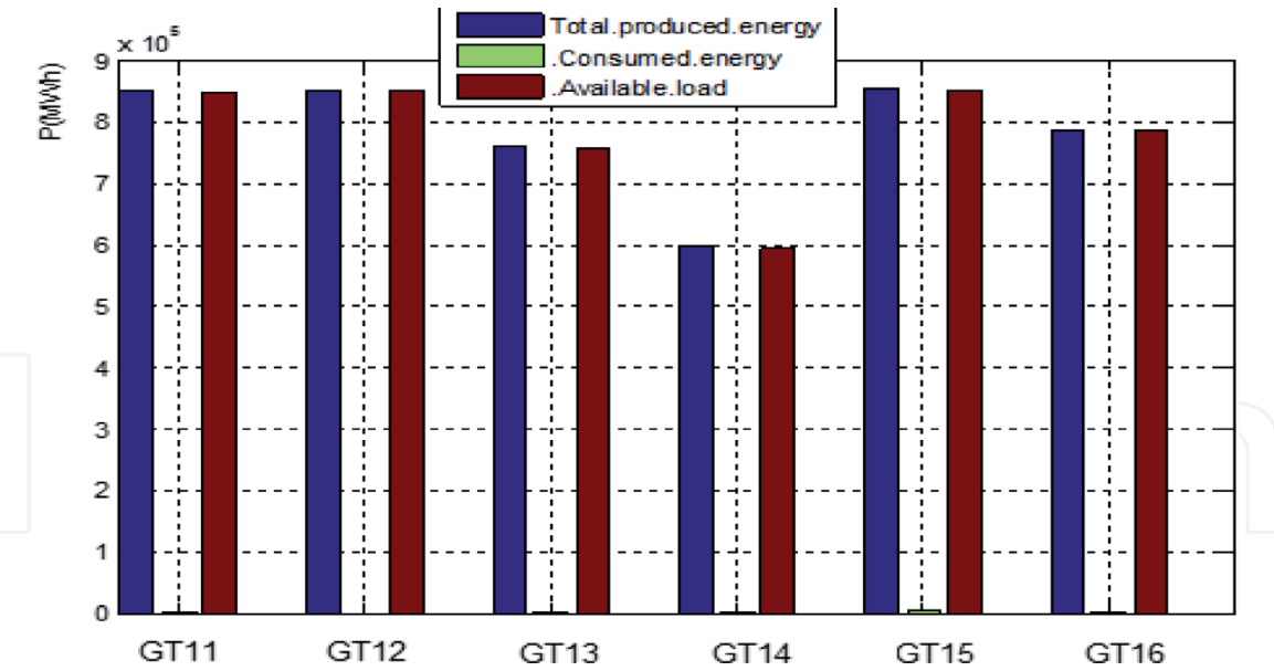
Figure 10. The total produced energy by the six units of the Western Mountain power plant in 2020.
