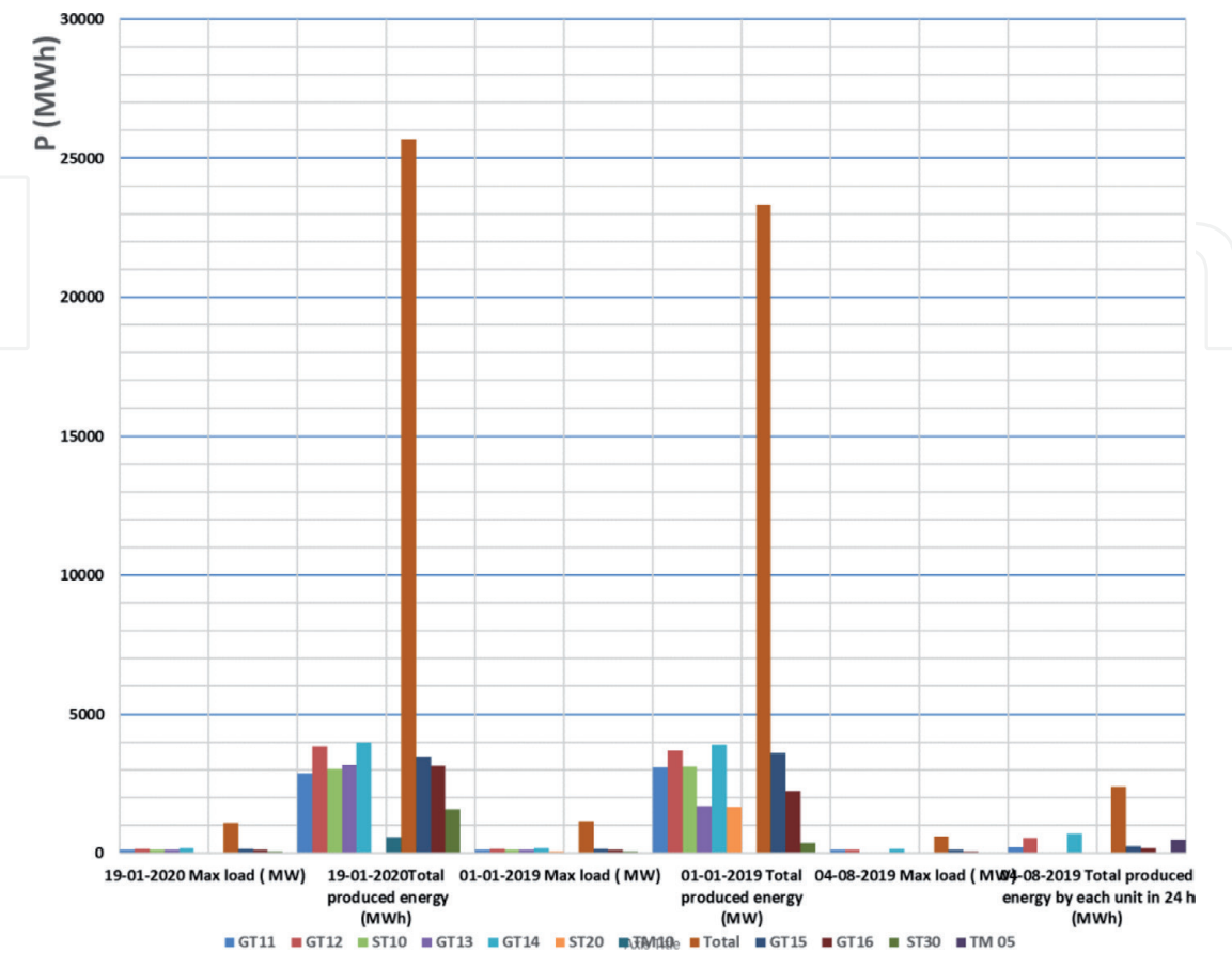
Figure 7. Comparative of the total produced energy on normal operation day and on the days of the blackouts.
