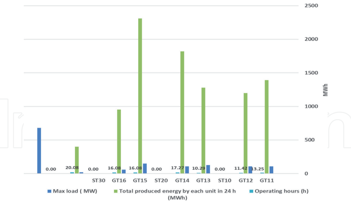
Figure 3. The produced energy by Al-Zawia CCPP on 02-08-2019.
