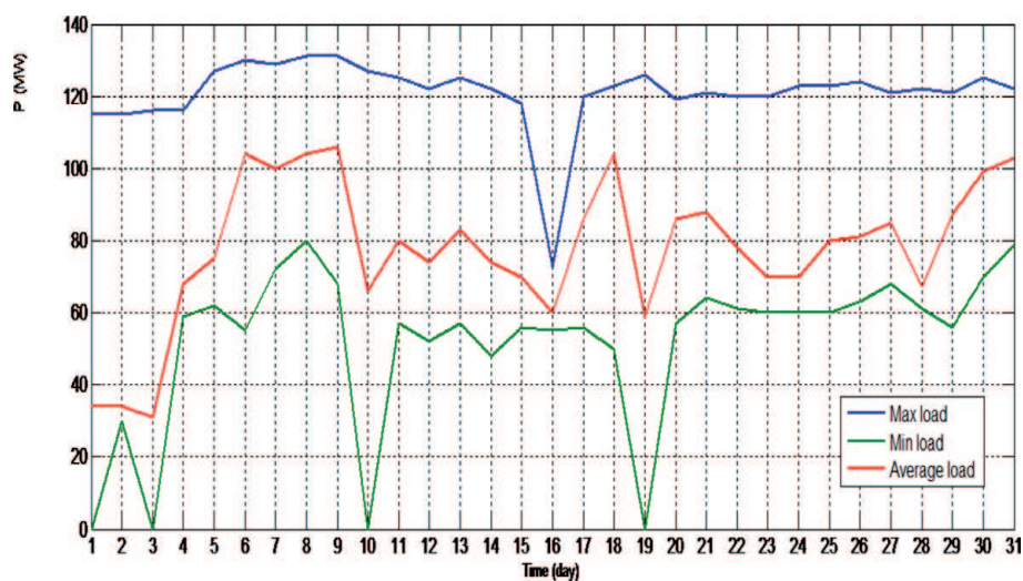
Figure 14. The performance of GT13 in Aug-2020.
