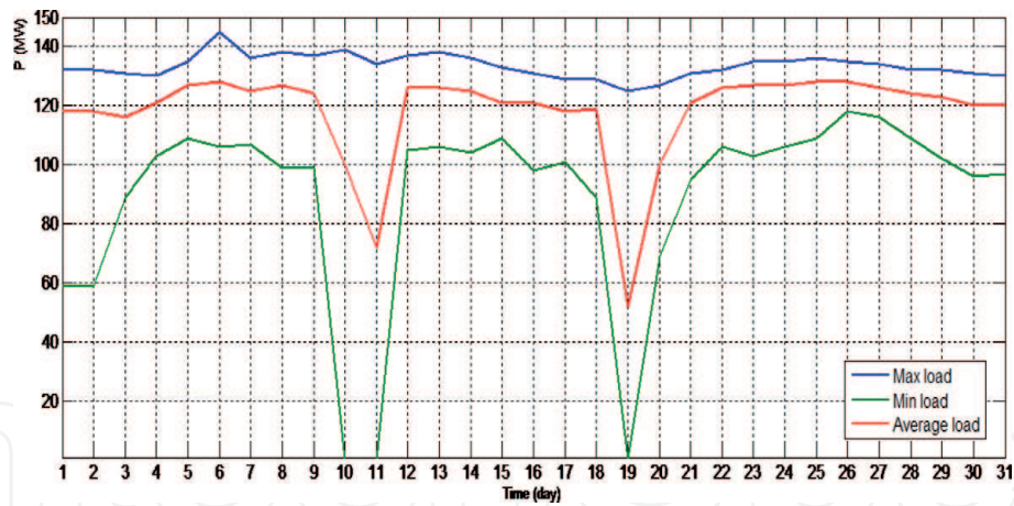
Figure 16. The performance of GT15 in Aug-2020.
