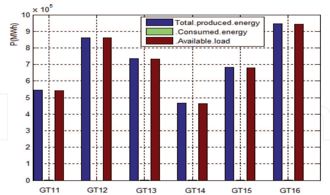
Figure 9. The total produced energy by the six units of the Western Mountain power plant in 2019.
