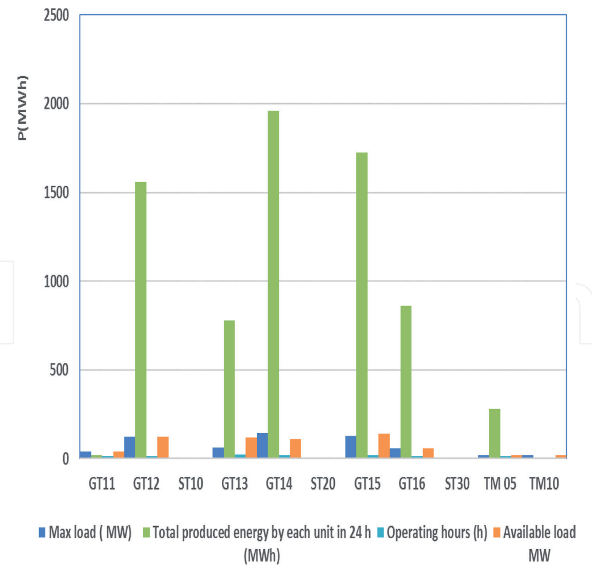
Figure 6. The performance of gas units of Al-Zawia CCPP on one day of the blackouts 07-08-2019.
