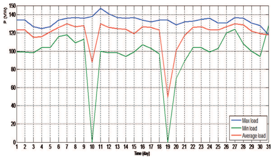
Figure 17. The performance of GT16 in Aug-2020.
