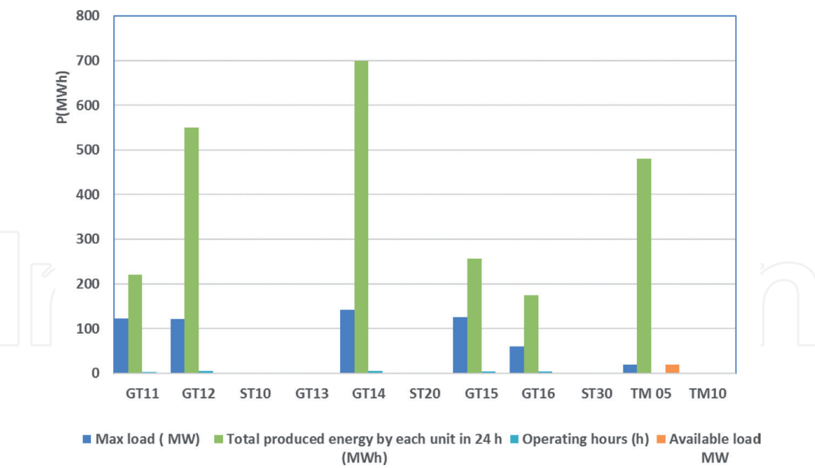
Figure 5. The produced energy by the units of Al-Zawia CCPP on of the day of the blackout 4-8-2019.
