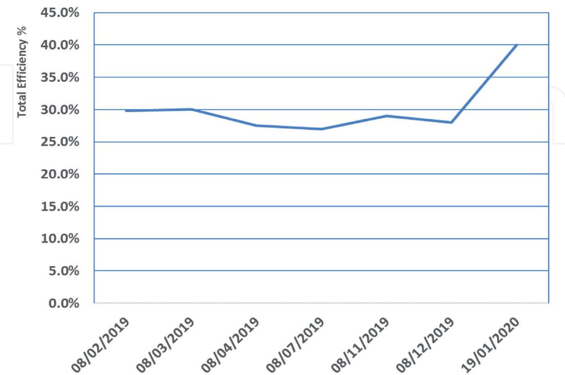
Figure 8. Comparative of the total efficiency on normal operation day and on the days of the blackouts.
