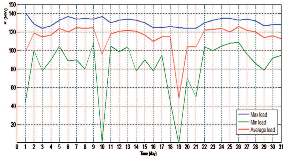
Figure 12. The performance of GT11 in Aug-2020.
