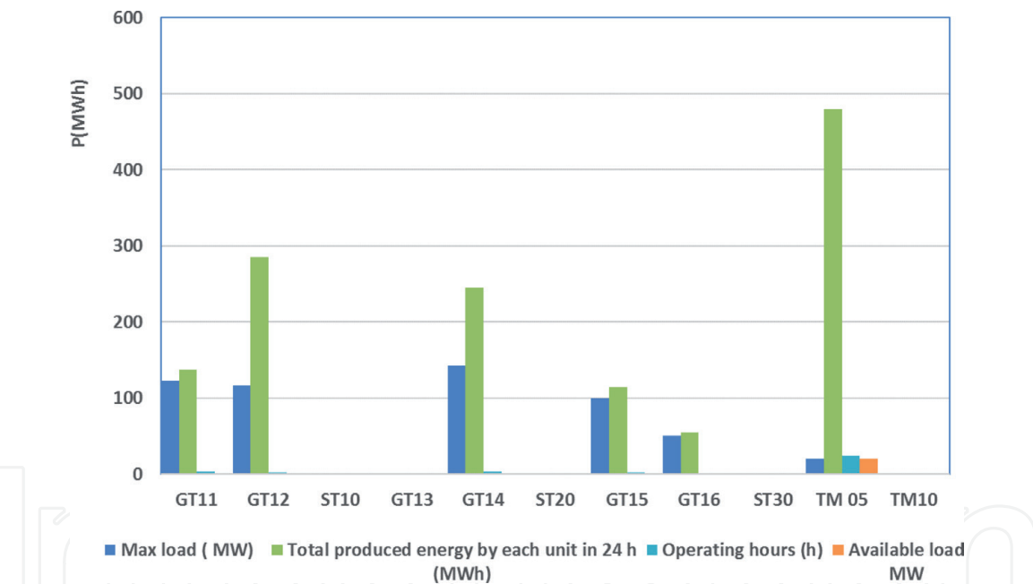
Figure 4. The statu of the nine units on the day of blackout 03-08-2019.
