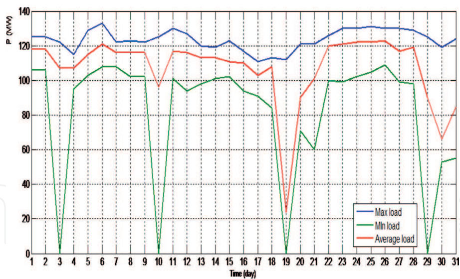
Figure 13. The performance of GT12 in Aug-2020.
