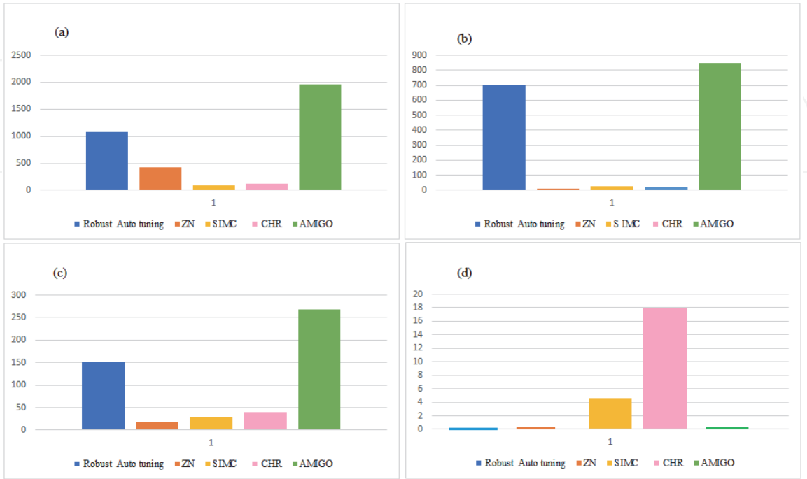
Figure 14. Comparative improvement time response specifications between tuning methods based OBT with respect to tuning lonely, (a)improvement td ratio, (b) improvement tr ratio, (c) improvement ts ratio, (d) improvement overshoot ratio.
