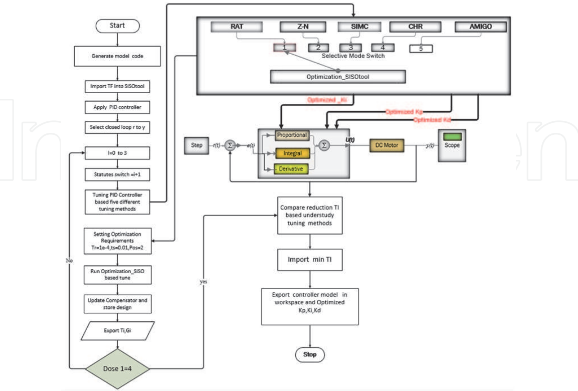
Figure 6. The PID controller based proposed technique.
