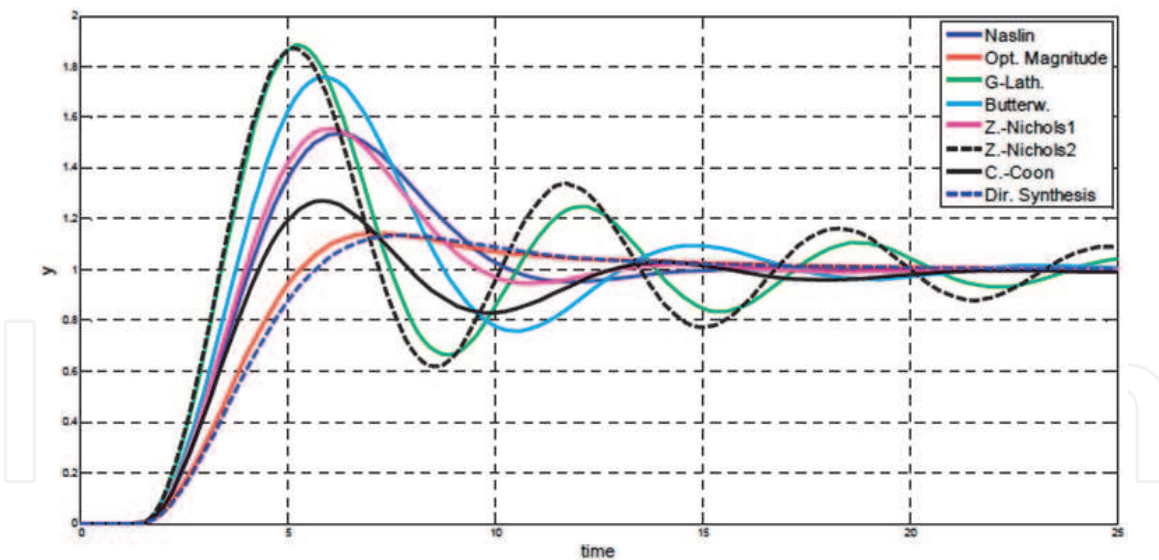
Figure 2. Time response specifications of PID controller under different classical tuning methods [24].
