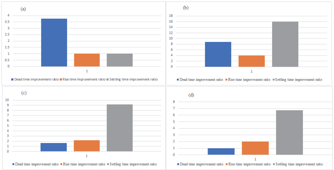
Figure 15. Comparative time response improvement ratio between AMIGO_{OBT} and other tuning methods based OBT , (a) improvement ratio comparing with RAT_{OBT} , (b) improvement ratio comparing with Z\_N_{OBT} , (c) improvement ts ratio comparing with SIMC_{OBT} , (d) improvement ratio comparing with CHR_{OBT} .
