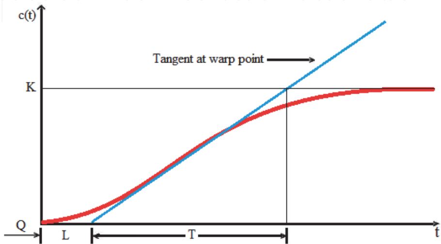
Figure 3. Step response of plant based Z-N tune [3].
