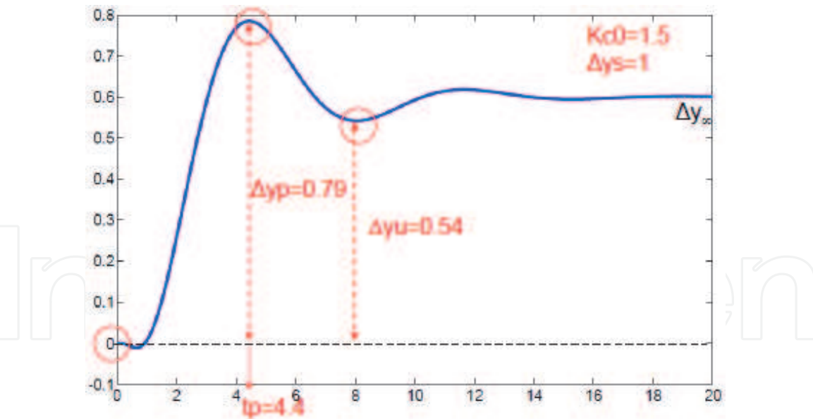
Figure 5. Extracting parameters from IMC closed-loop set point response with PID controller [20].
