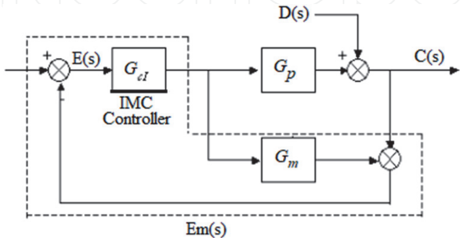
Figure 4. IMC structure [6].
