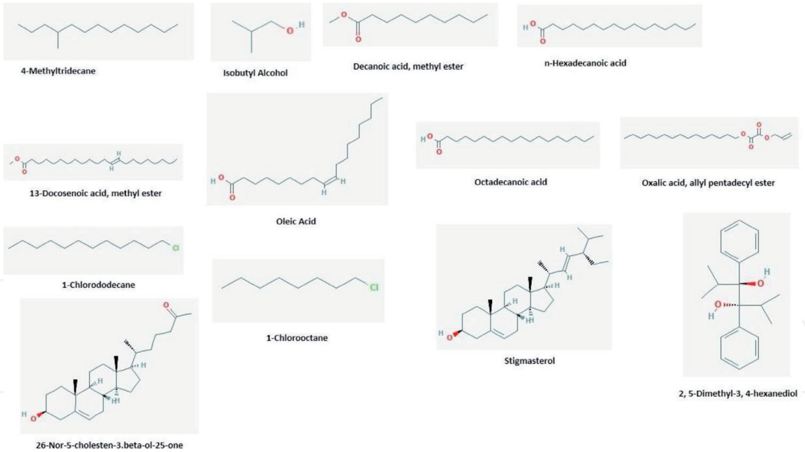
Figure 8. Chemical structures of Identified Bioactive compounds from Antheraea mylitta Cocoon Extract.
