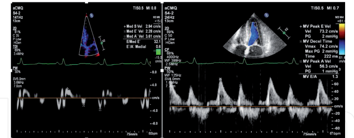
Figure 4. 2D echocardiogram with tissue Doppler sample at base of the interventricular septum and pulsed-wave Doppler at mitral valve inflow in a patient with AL type cardiac amyloidosis revealing impaired relaxation, septal e' of the LV decreased and a pseudonormal pattern.
