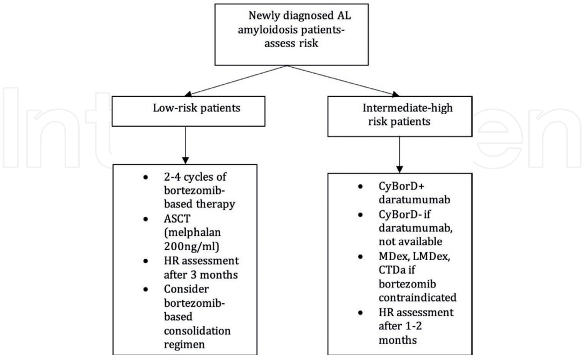
Figure 8. Treatment algorithm of AL Amyloidosis. CyBorD = cyclophosphamide and dexamethasone; ASCT = autologous stem cell transplantation; MDex = melphalan and dexamethasone; LMDex = lenalidomide, melphalan, and dexamethasone; CTDa = cyclophosphamide and dexamethasone; HR = heart rate.
