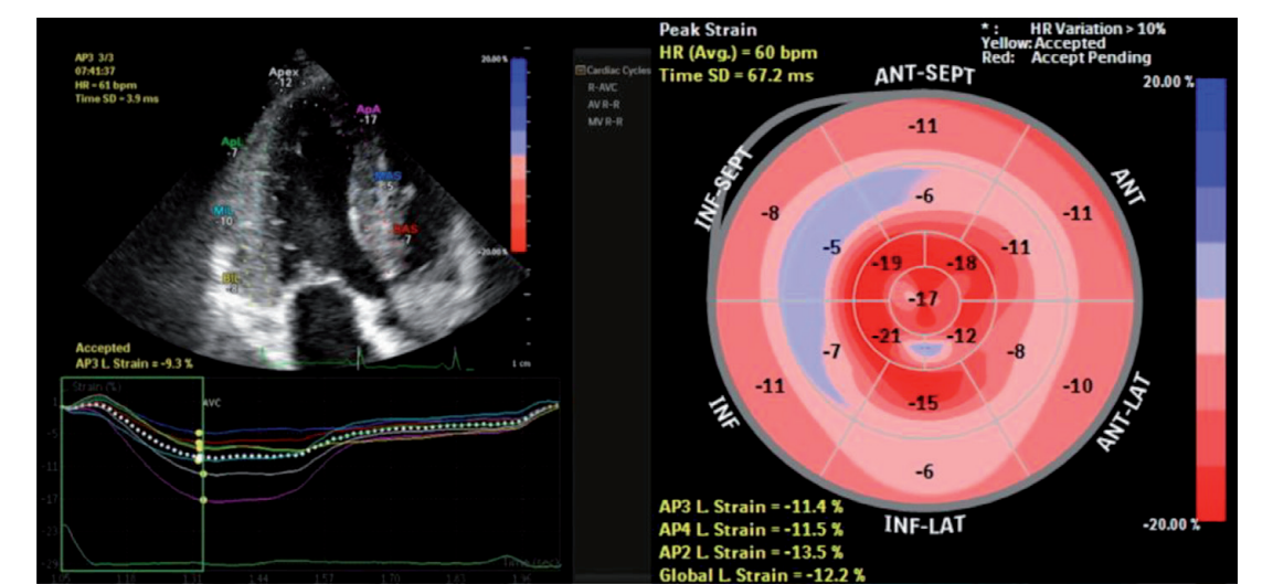
Figure 5. Left ventricular strain image with impaired longitudinal shortening at basal and mid-ventricular level with preserved longitudinal function at the apex (relative apical sparing) as seen in the bull's eye plot on the right.
