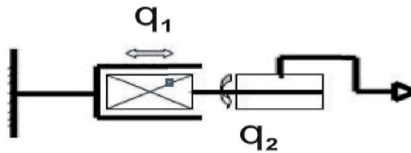
Figure 2. Kinematic scheme of the mechanical structure.
