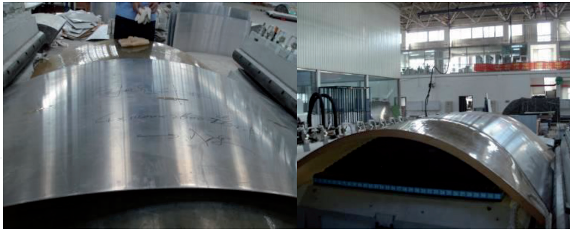
Figure 14. Skin drawing based on flexible multi-point die.
