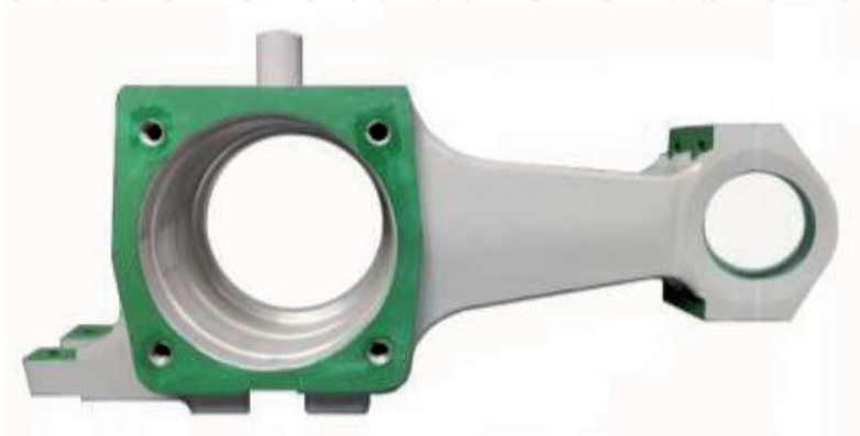
Figure 11. Finished aluminum alloy axle box of high-speed train.
