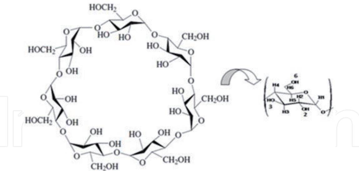
Figure 3. βCD molecule [29].
