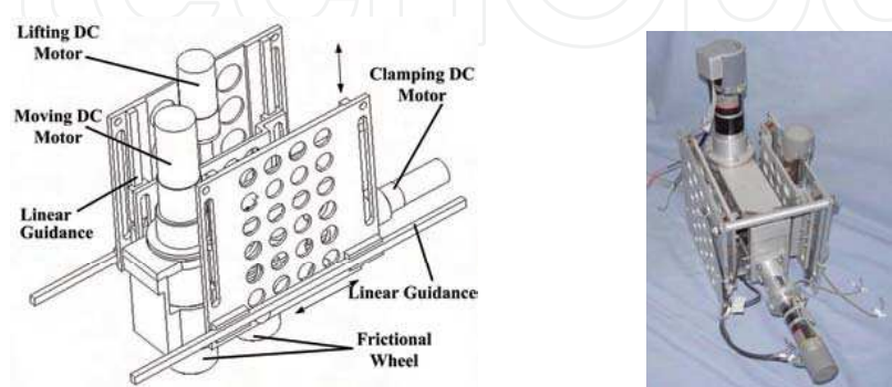
Fig. 9. Mechanical structure of the wheel set.
