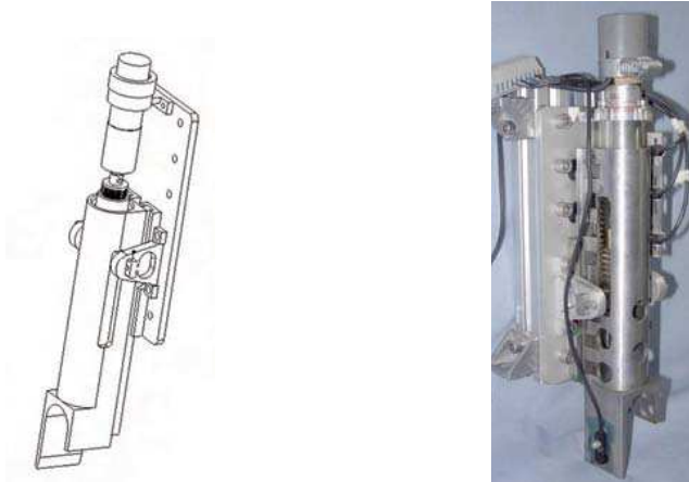
Fig. 7. The clutch mechanism.
