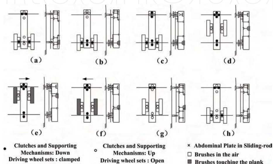
Fig. 17. Cleaning movement.
