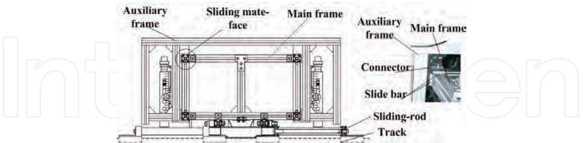
Fig. 6. Sliding-mate between two frames.
