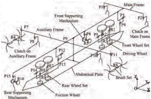
Fig. 3 Mechanical construction of the robot.
