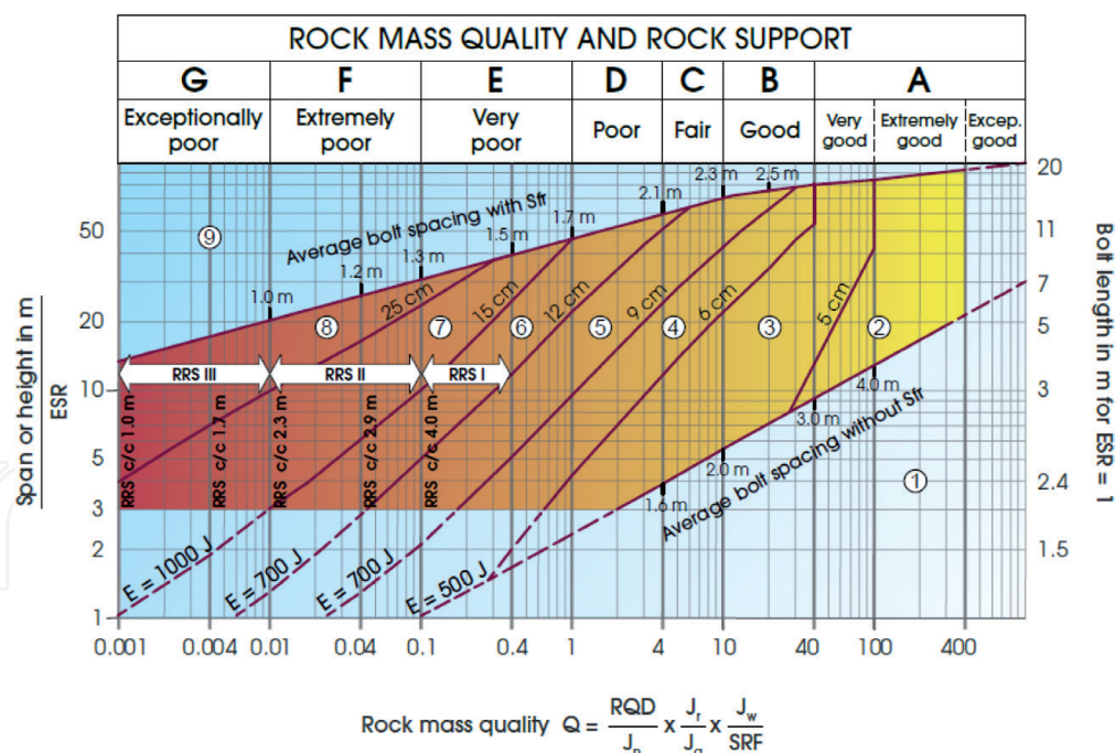
Figure 2. Tunnel support chart based on Q-system [2].
