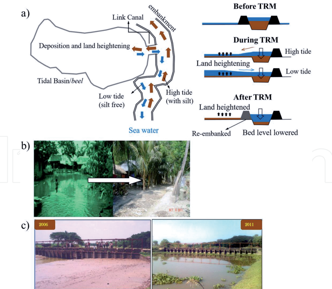
Figure 4. (a) Tidal basin concept: Free play of tidal flow in selected beel, (b) land reclamation in Arua village in between 2005 and 2011 [11], and (c) revival of Hari River near Bhabodah regulator in between 2006 and 2011 [14] (adapted from Talchabhadel et al., [8]).
