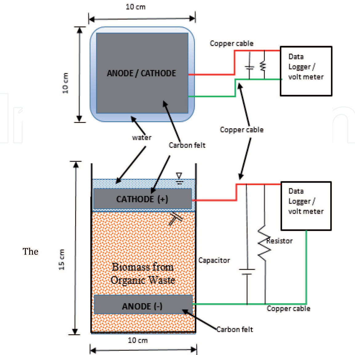
Figure 1. Schematic diagram of the MFC used in the laboratory.
