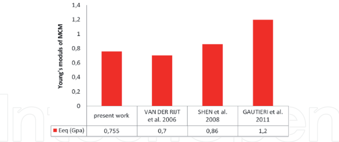
Figure 10. Comparison between NN predicted average Young's modulus of MCM and literature results [7].
