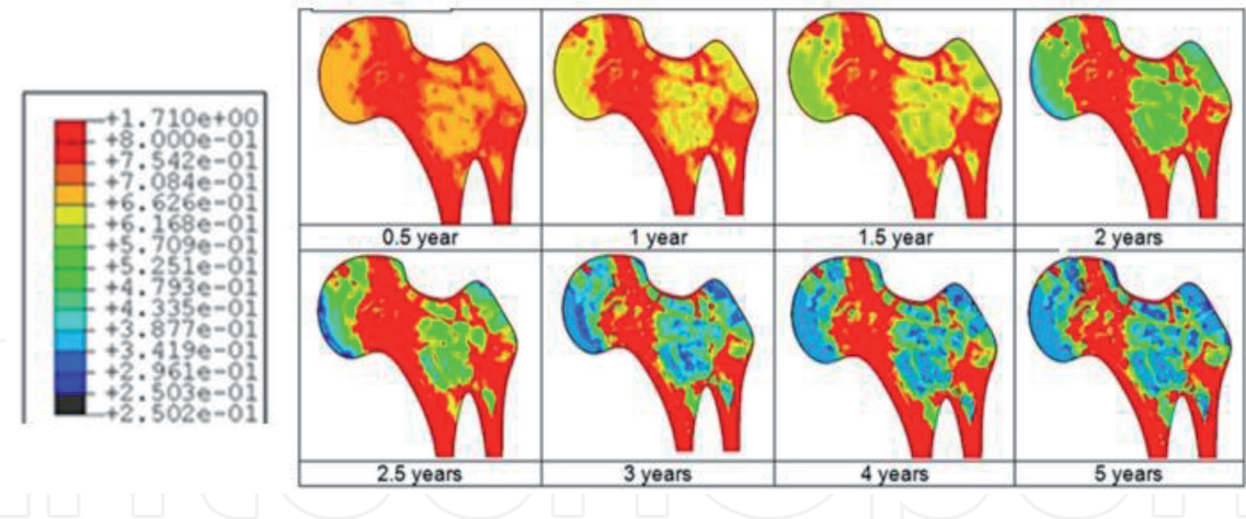
Figure 12. Predicted bone adaptation sequences in the form of apparent bone density variation in gram per cubic centimeter [18].
