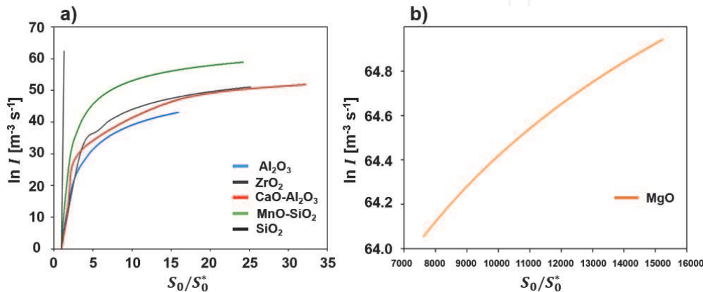
Figure 4. Effect of supersaturation ratios on nucleation rate at 1600°C, (a) various metal deoxidizers, (b) with magnesium.
