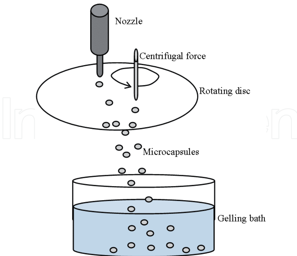
Figure 6. Schematic representation of the spinning disc assembly.
