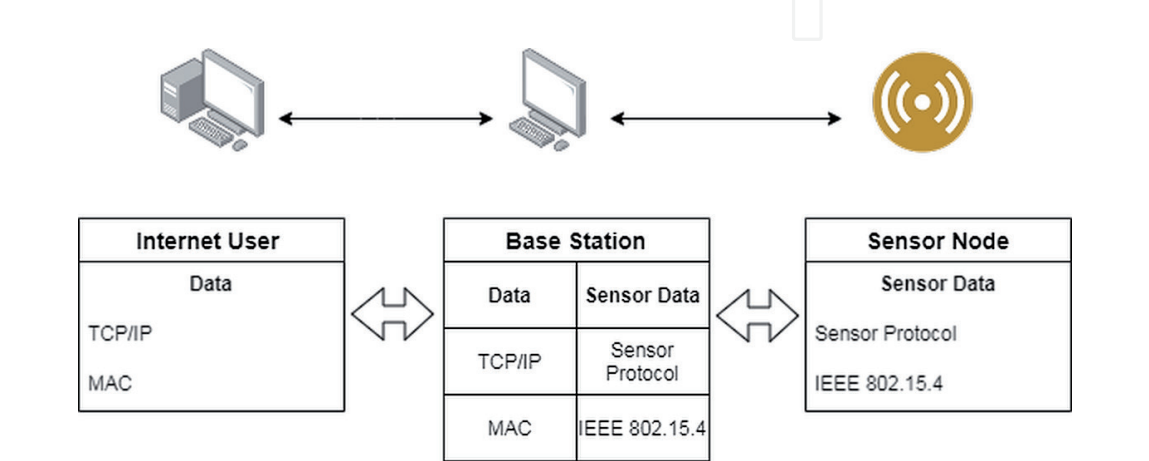
Figure 6. Front end proxy solution.
