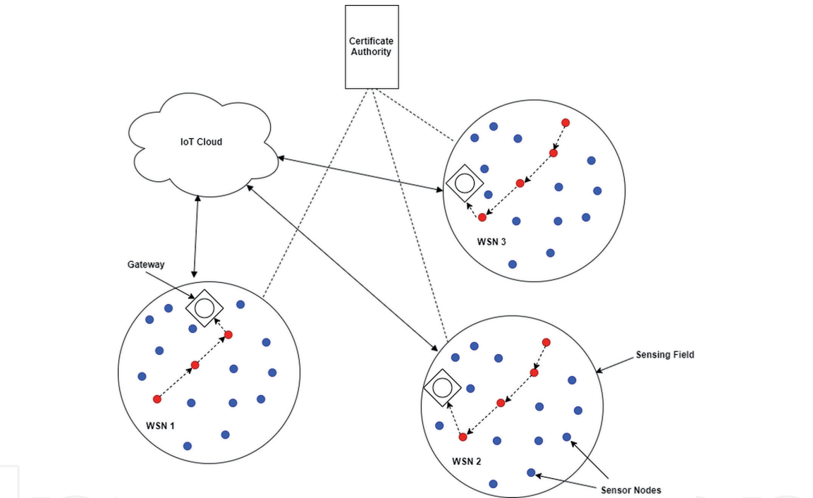
Figure 4. IoT architecture.
