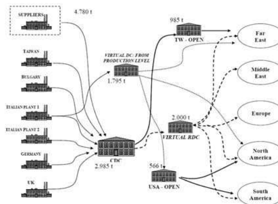
Figure 11. Multi-commodity model
