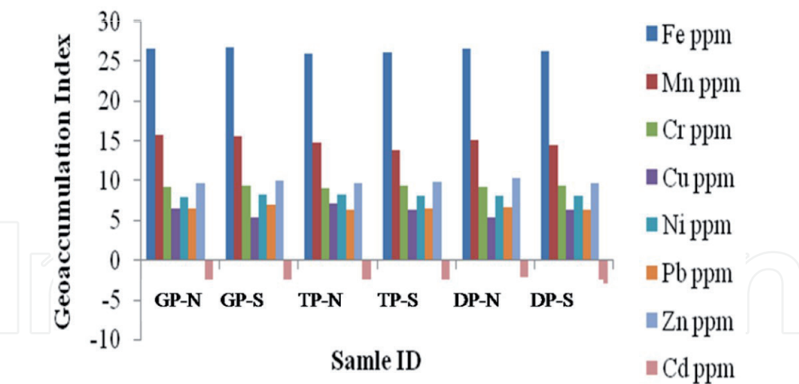
Figure 7. Graphical representation of Igeo for heavy metals.
