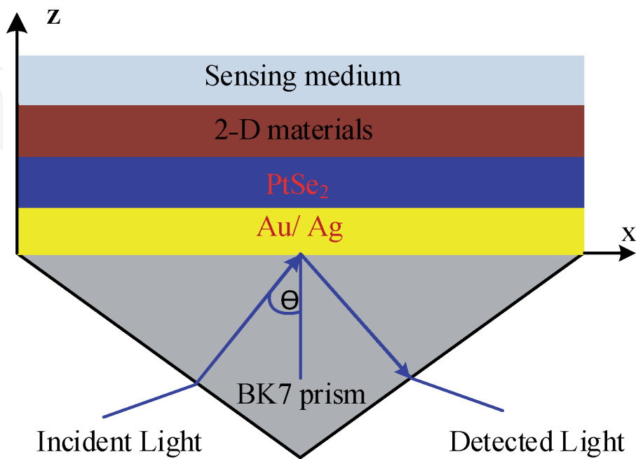
Figure 4. Schematic Illustration of SPR biosensor employing hybridization of 2D materials with Ag/Au [86].
