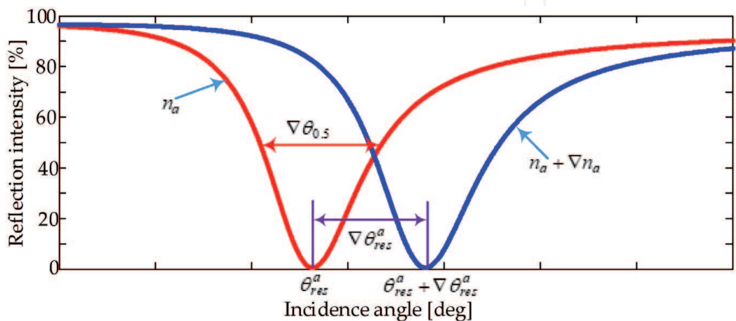
Figure 3. Illustration of the SPR curve variation due to change in sensing medium RI.
