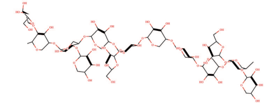
Figure 4. Three-dimensional representation of the heteroxylan present in Scheelea phalerata (Uricuri) palm gum, with \beta\text{-(1}\rightarrow 4) bonds. Main chain branches are substituted at O-2 or O-3 positions by arabinose and xylose units.
