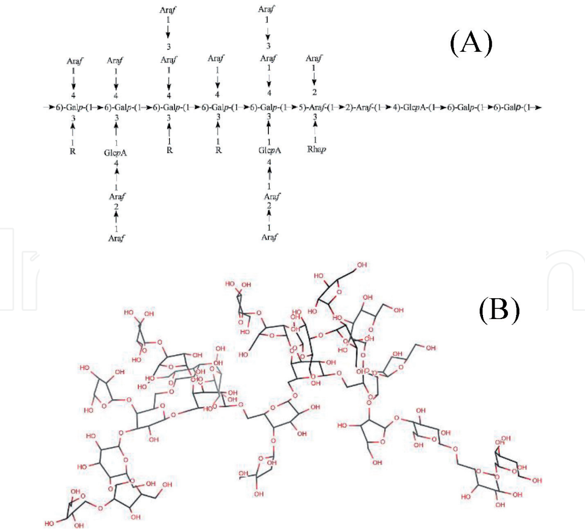
Figure 2. Structural fragment of gum ghatti. (A) Scheme and (B) three-dimensional structure referring to the fragment shown.
