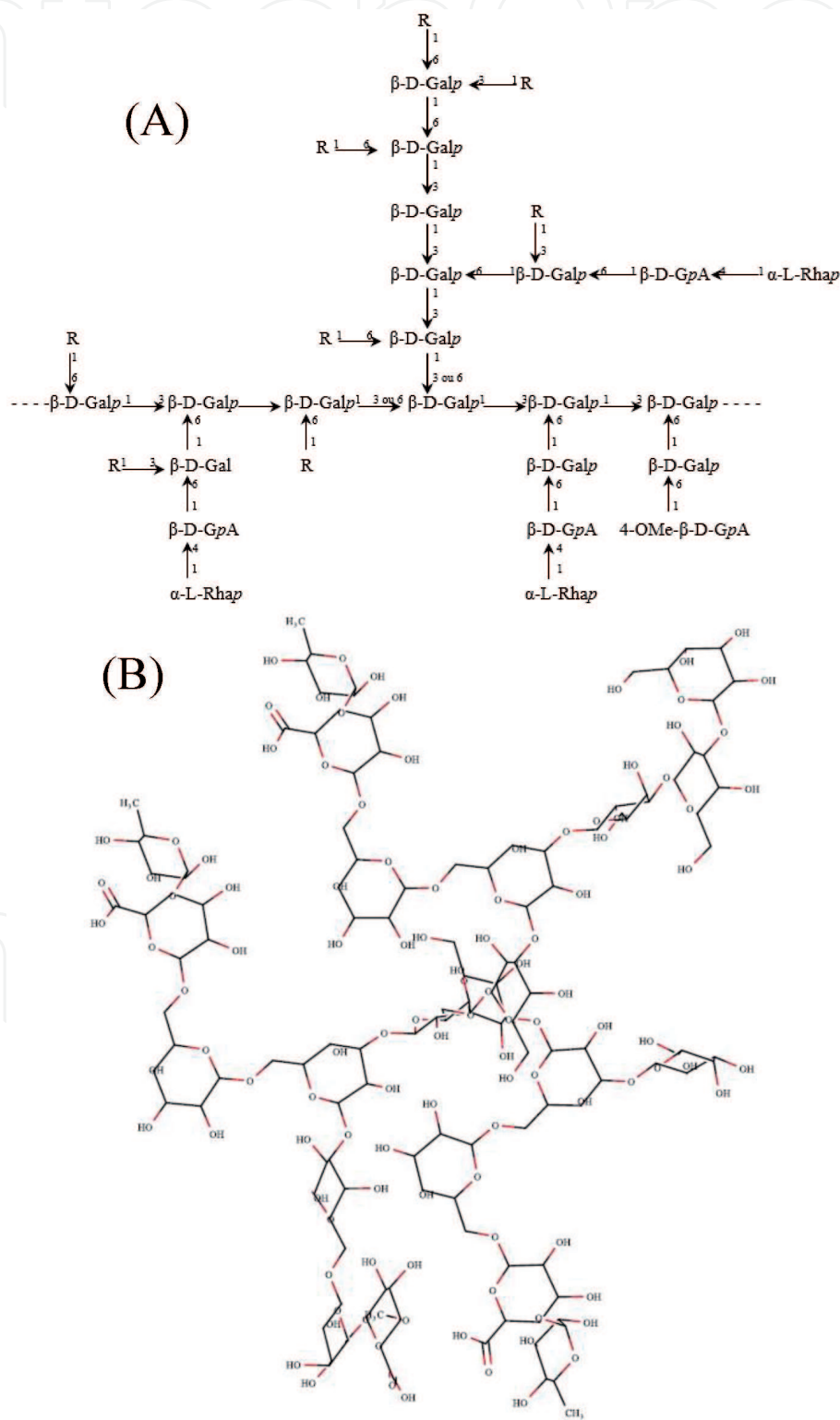
Figure 1. Structural fragment of gum arabic ( Acacia senegal ). (A) Scheme and (B) three-dimensional structure referring to the fragment shown.
