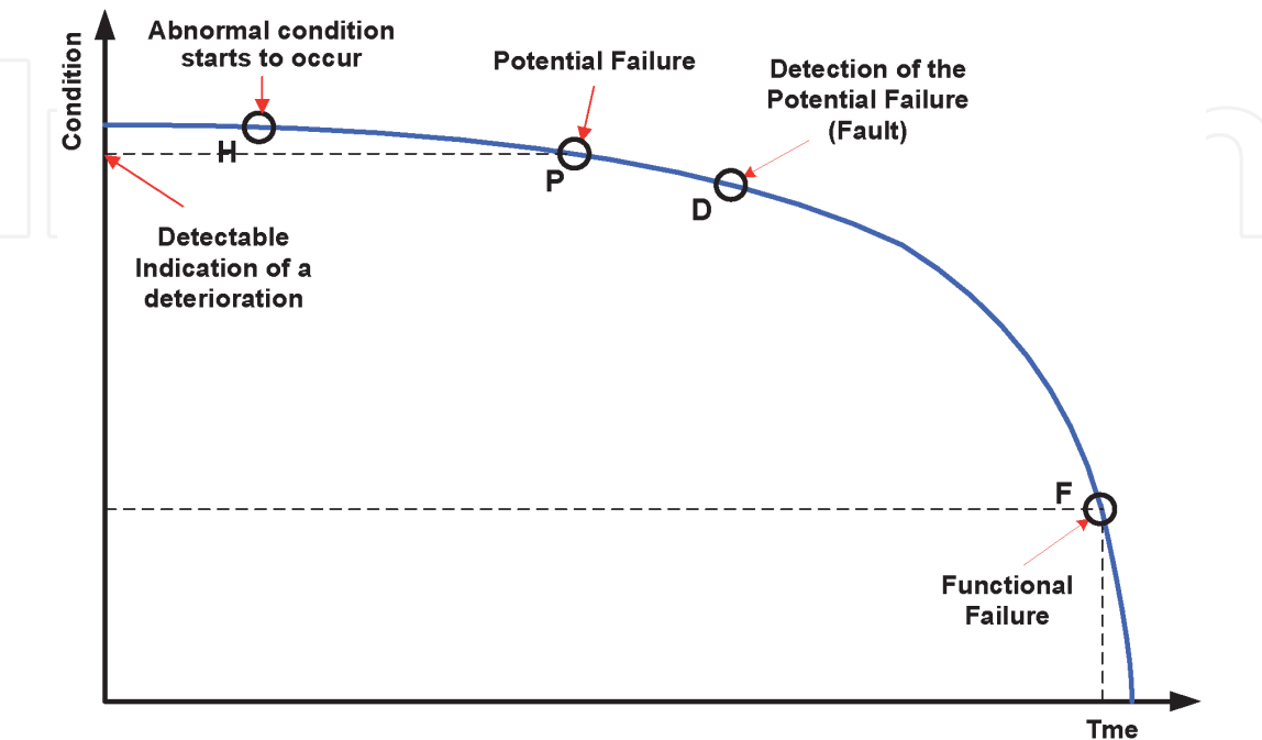
Figure 12. Equipment failure mode diagram (adapted from [19]).
