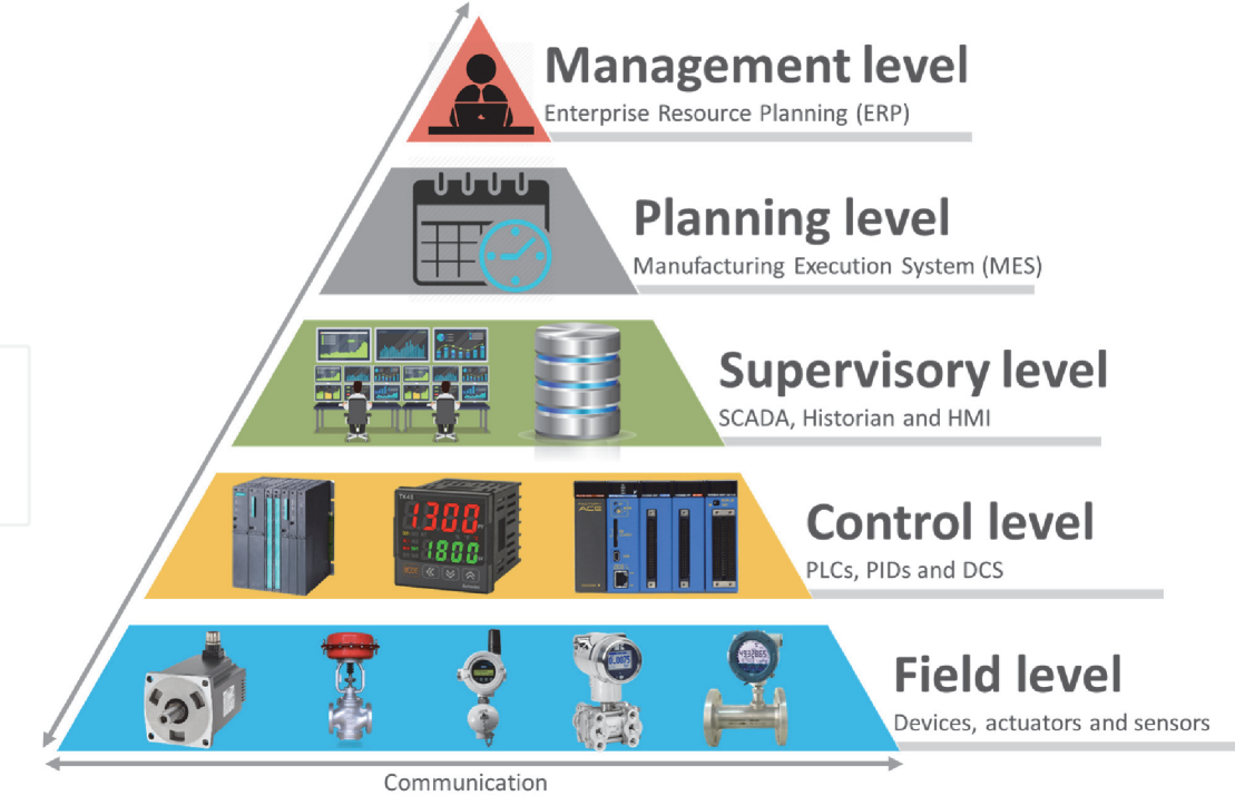
Figure 1. The automation pyramid of a typical industrial plant.
