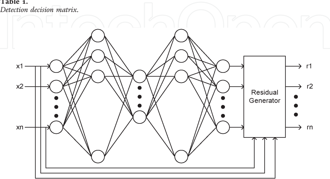
Figure 14. Architecture of an AANN for anomaly detection.
