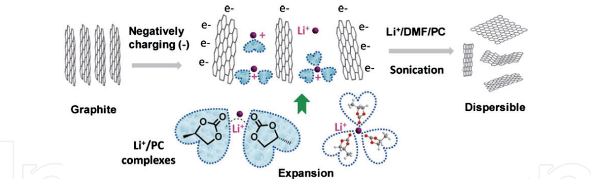
Figure 6. Exfoliation of graphite into few-layer graphene flakes via intercalation of Li + complexes [44].
