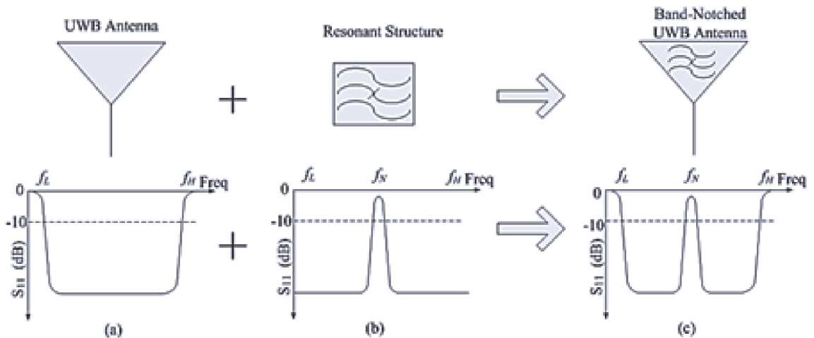
Figure 2. The basic design of UWB antenna with band-notched characteristic: (a) UWB antenna, (b) Band-notch resonant structure and (c) Band-notched UWB-antenna.
