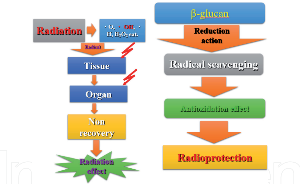
Figure 7. Radiation protection and radical scavenger processes.
