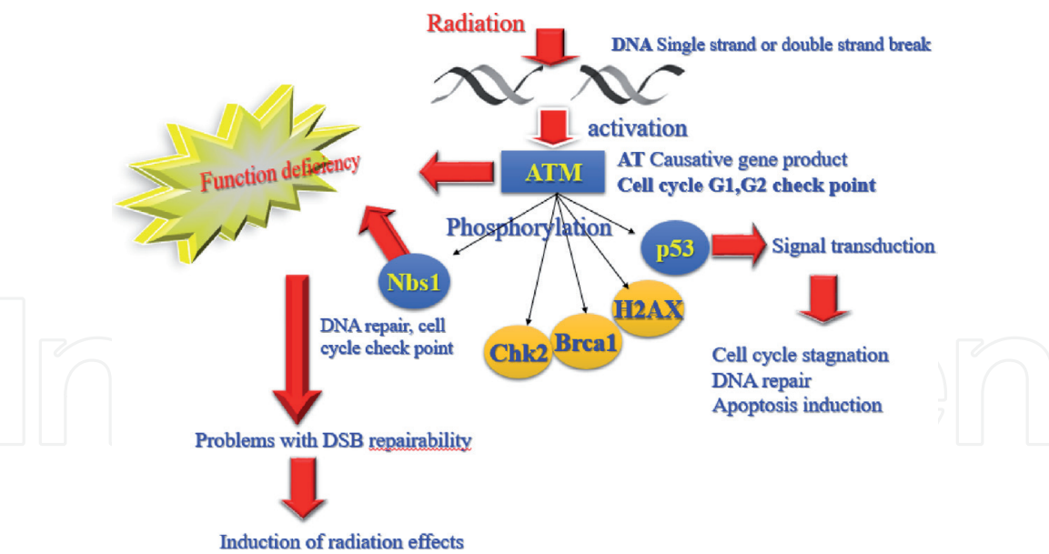
Figure 6. Mechanisms of cell repair in radiation protection.
