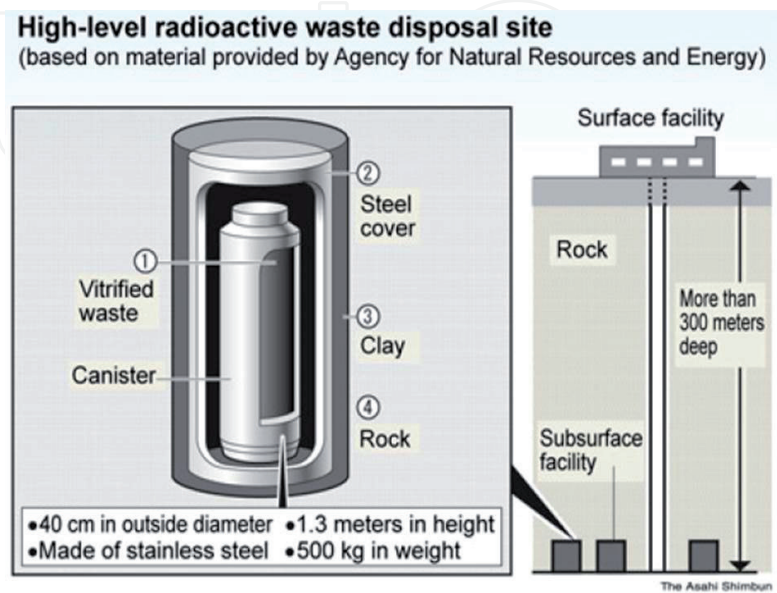
Figure 4. Deep well disposal method.
