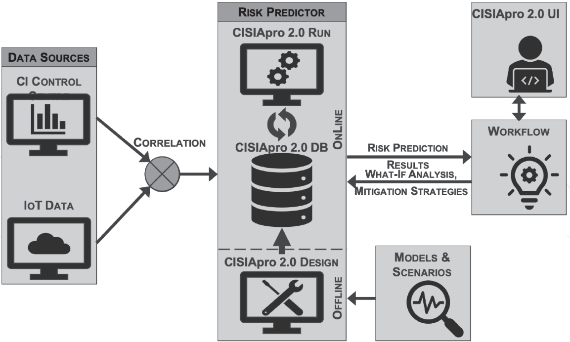
Figure 5. CISIApro 2.0 architecture.
