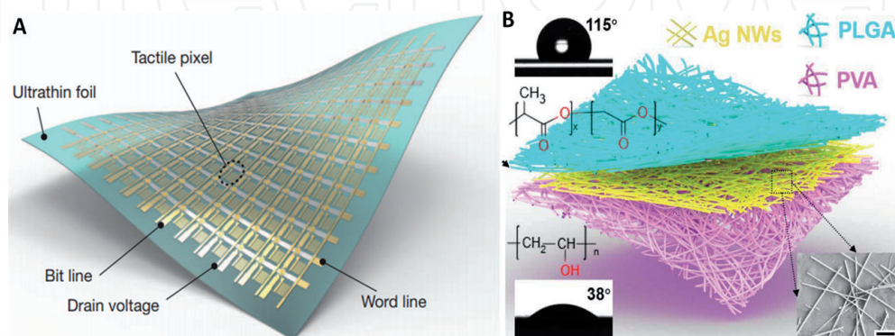
Figure 8. (A) Illustration of a thin large-area active-matrix sensor with 12 \times 12 tactile pixels. Adapted from Ref. [63]. (B) Schematic illustration of the three-dimensional network structure of the all-nanofiber TENG-based e-skin. The images of the water contact angle and molecular structure of PLGA and PVA are inserted on the top left and lower left, respectively. The surface SEM image of the Ag NW electrode is inserted on the lower right (scale bar, 2 \mu\text{m} ). Adapted from Ref. [68].
