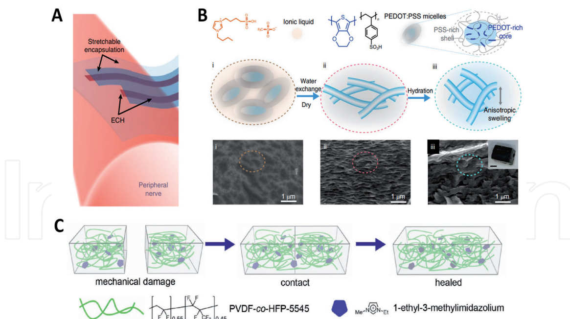
Figure 11. (A) Schematic of the bioelectronic interface between a peripheral nerve and soft conductor electrodes and insulation materials. (B) Schematic of the stepwise PEDOT:PSS ECH synthesis process and SEM images showing morphological changes in each step during the synthesis of an ECH. An ionic liquid, 4-(3-butyl-1-imidazolium)-1-butananesulfonic acid triflate, was blended with the PEDOT:PSS solution and subsequently dried to form an ion gel (i); ionic liquid is exchanged with water and then dried at room temperature (ii); the dried sample exhibits aligned and interconnected microstructures that swell in water to form the ECH (iii). The interconnected PEDOT polymer network in the ECH results in a continuous electronic conductive pathway. Scale bar, 1 mm for the inset of (iii), which is an optical image of a hydrated ECH. Adapted from Ref. [88]. (C) Design concept for a transparent, self-healing, highly stretchable ionic conductor using ion-dipole interaction as the dynamic motif and demonstration of healing process and chemical structure of polymer and imidazolium cation. Adapted from Ref. [89].
