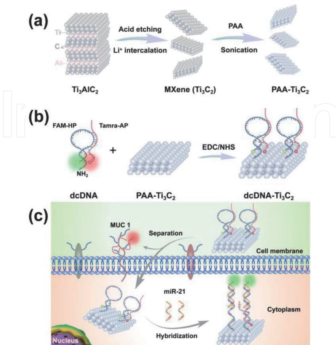
Figure 4. (a) Illustration of the fabrication of the \text{Ti}_3\text{C}_2 MXenes and PAA- \text{Ti}_3\text{C}_2 . (b) the construction of the dcDNA- \text{Ti}_3\text{C}_2 composite nanoprobe. (c) Multilayer imaging of plasma membrane glycoproteins MUC1 and cytoplasmic miR-21 using the dcDNA- \text{Ti}_3\text{C}_2 composite nanoprobe. Reprinted with permission from ref. [128]. Copyright ACS, 2019.
