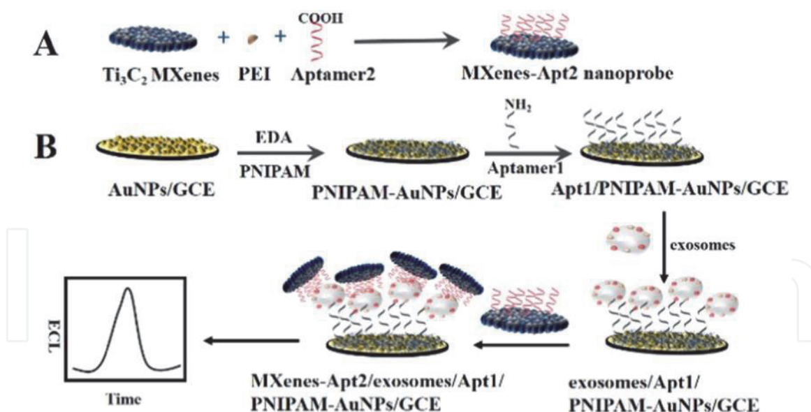
Figure 5. The principle of the ECL biosensor for exosomes activity detection signal amplification strategy. Reprinted with permission from Ref. [134]. Copyright ACS, 2018.
