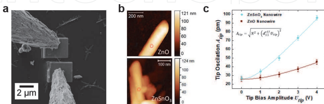
Figure 6. (a) SEM image showing the tungsten tips of the nanomanipulators, which are contacting in-situ deposited Pt electrodes for the electrical characterization of a single \text{ZnSnO}_3 nanowire. Atomic force microscopy characterization of individual ZnO and \text{ZnSnO}_3 nanowires: (b) topographies in noncontact mode, and (c) contact mode tip oscillation as a function of tip-bias ac-voltage. Reprinted with permission from [63]. Copyright 2020 American Chemical Society.
