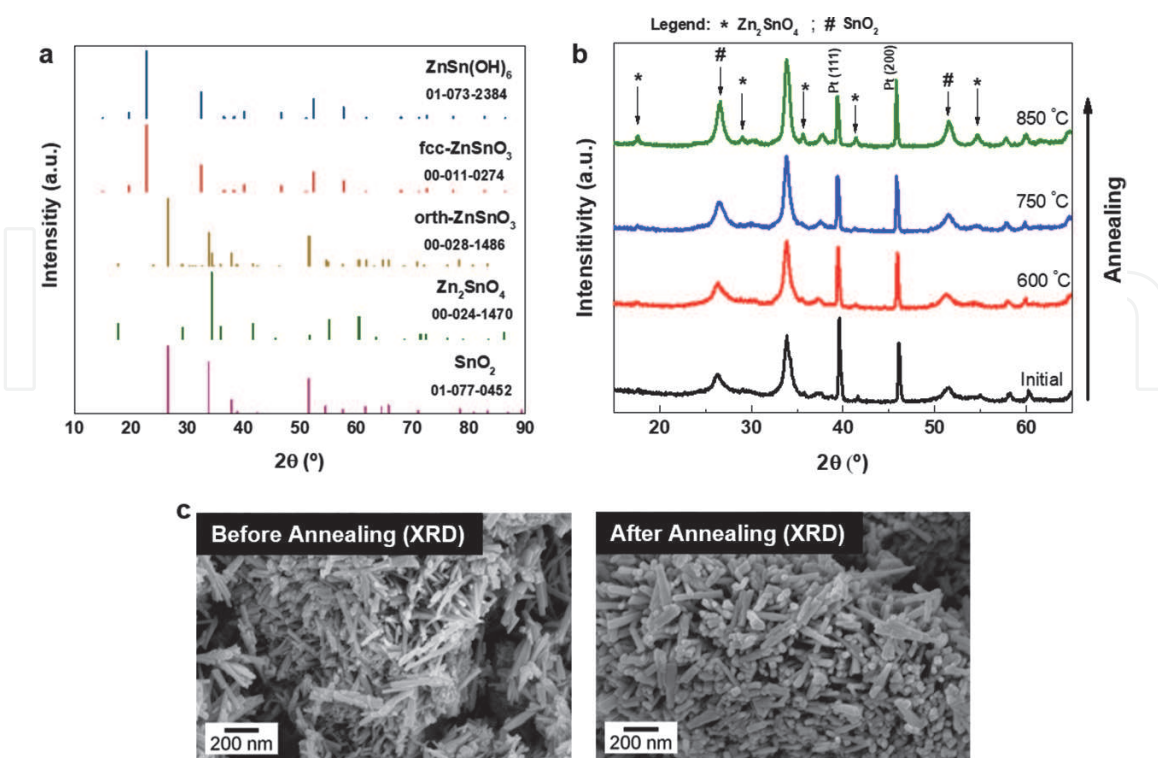
Figure 4. (a) Representation of XRD peaks of ICDD cards of: \text{ZnSn}(\text{OH})_6 , fcc- \text{ZnSnO}_3 , orth- \text{ZnSnO}_3 , \text{Zn}_2\text{SnO}_4 and \text{SnO}_2 . Note that the card 00-028-1486 (orth- \text{ZnSnO}_3 ) was deleted from ICDD. (b) In-situ XRD patterns of \text{ZnSnO}_3 nanowires during annealing until 850°C. (c) SEM images of the \text{ZnSnO}_3 nanowires before and after the in-situ annealing experiments in XRD.
