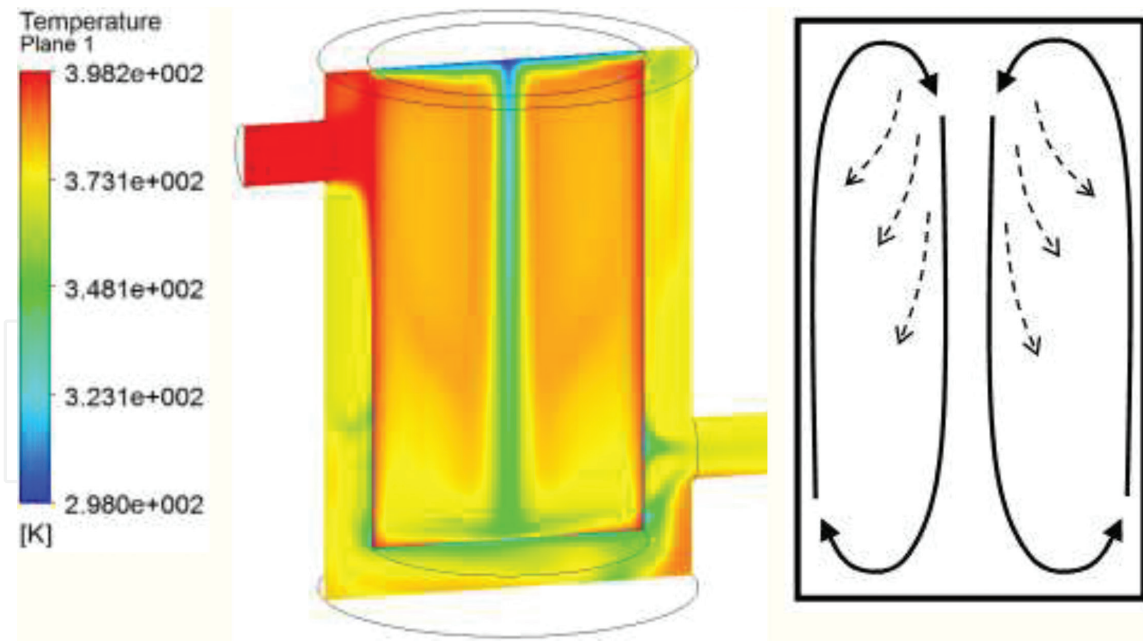
Figure 4. Thermal profile in vertical plane for the two simulated domains showed simultaneously and the simplified scheme of the primary (continuous) and secondary (dashed) heat fluxes inside reaction vessel after the formation of natural convection cell.
