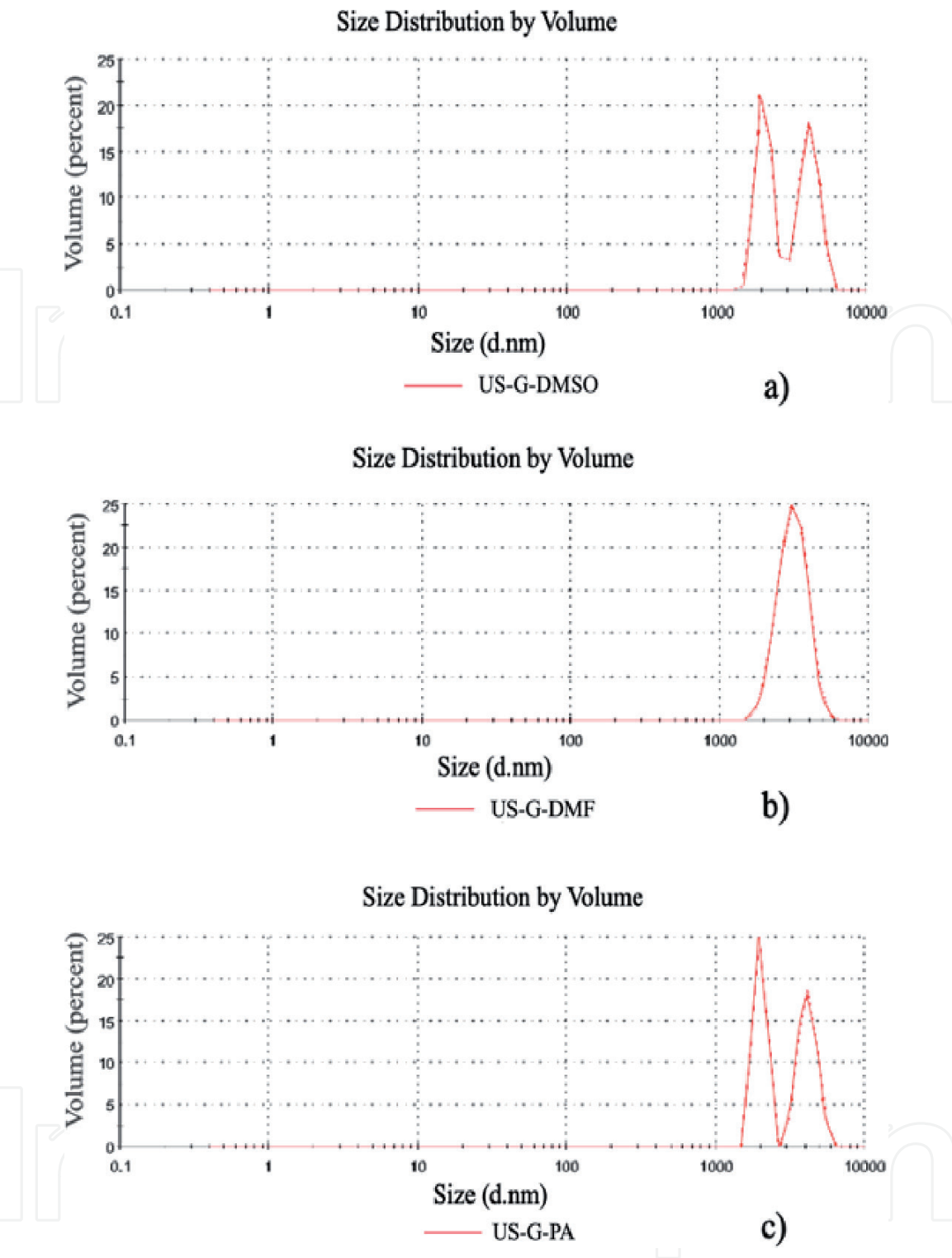
Figure 13. Lateral size results of synthesized samples, (a) US-G-DMSO, (b) US-G-DMF, (c) US-G-PA.
