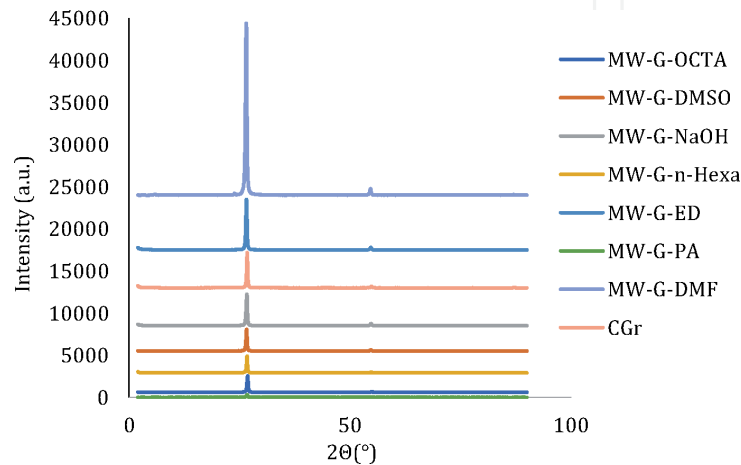
Figure 9. XRD spectra of MW-assisted graphene products.
