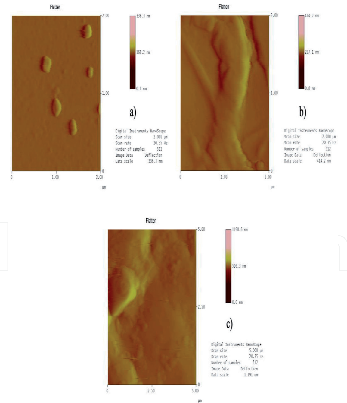
Figure 12. The AFM images of (a) US-G-DMSO, (b) US-G-DMF, and (c) US-G-PA drop casted onto glass piece showing the homogeneous structure of the pristine graphene nanosheets.
